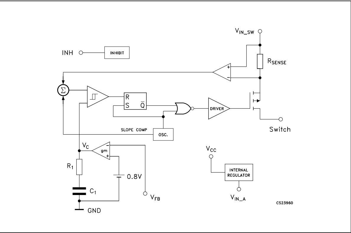
Figure 1. Schematic diagram
