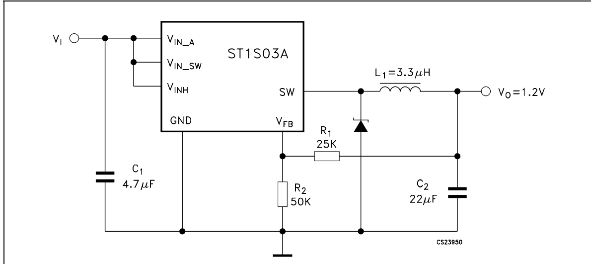
Figure 3. Application circuit
