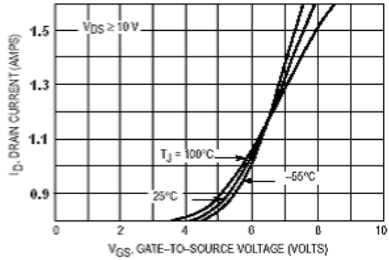
Figure 2. Transfer Characteristics
