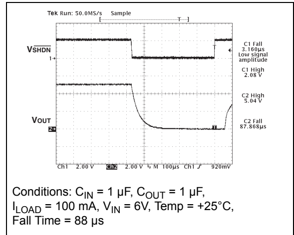
FIGURE 2-22: Measure Fall Time of 5.0V LDO.
