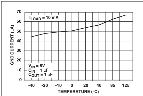
FIGURE 2-14: GND Current vs. Temperature ( I_{LOAD} = 10 mA ).
