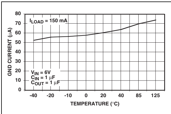
FIGURE 2-15: GND Current vs. Temperature ( I_{LOAD} = 150 mA ).
