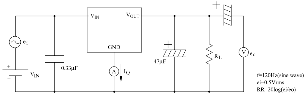
Fig. 4 Ripple Rejection Test Circuit (Fixed-Type)
