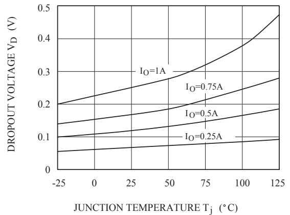
Fig.8 T_j - V_D
