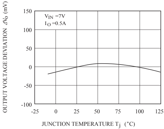
Fig.5-1 T_j - \Delta V_O (KIA78R05)
