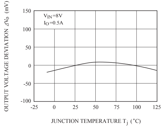
Fig.5-2 T_j - \Delta V_O (KIA78R06)
