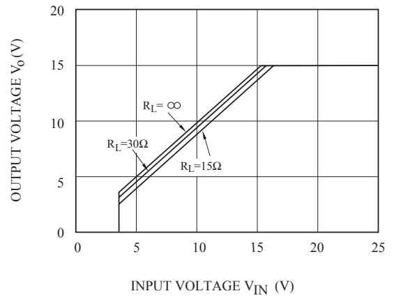
Fig.6-7 V_{IN} - V_o (KIA78R15)
