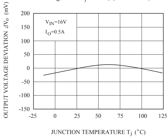
Fig.5-5 T_j - \Delta V_o (KIA78R10)
