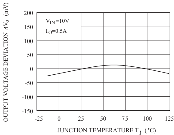
Fig.5-3 T_j - \Delta V_O (KIA78R08)
