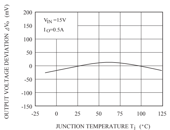
Fig.5-4 T_j - \Delta V_O (KIA78R09)
