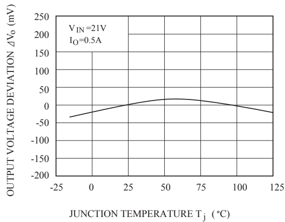
Fig.5-7 T_j - \Delta V_o (KIA78R15)
