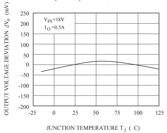
Fig.5-6 T_j - \Delta V_o (KIA78R12)
