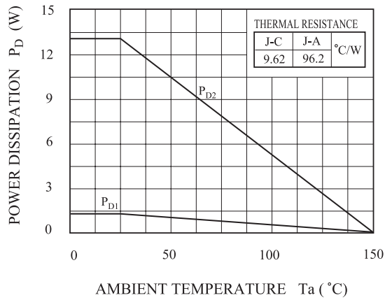
Fig.11 P_D - T_a (F-Type : DPAK-5)
