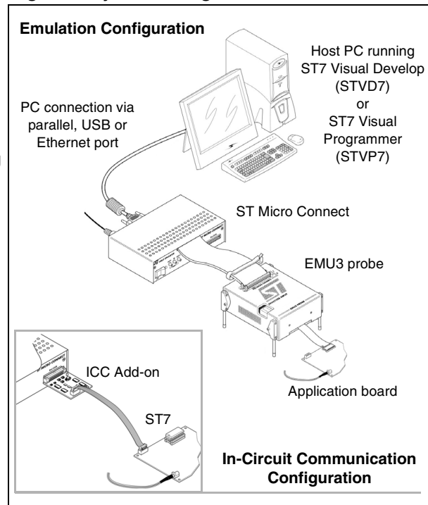
Figure 1: System configurations
