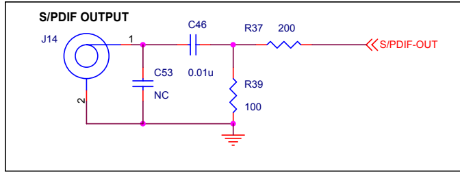
S/PDIF Output Connection option 1: Coaxial
