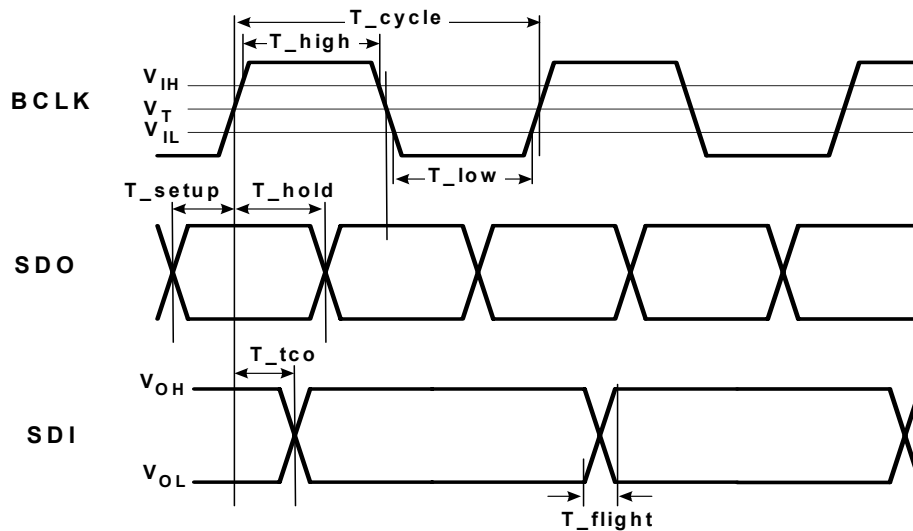
Figure 16. Link Signal Timing
