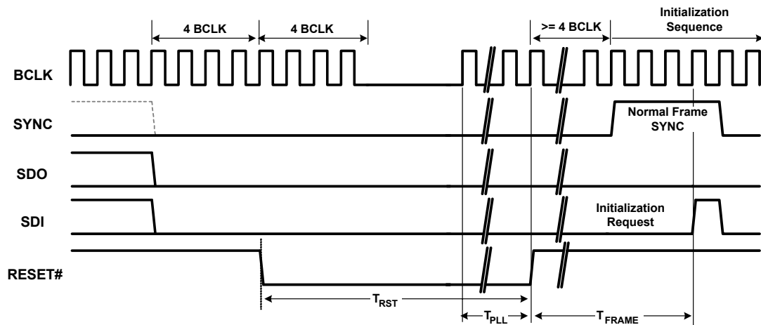
Figure 15. Link Reset and Initialization Timing
