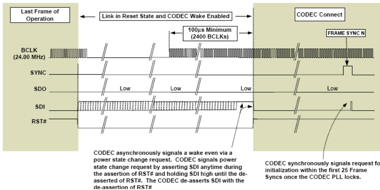
Figure 14. Resume From External Event (Wake-Up Event)
