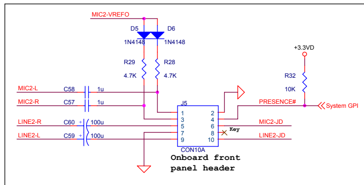
Option 1: MIC2 (port-F) and LINE2 (port-E) to front panel header
