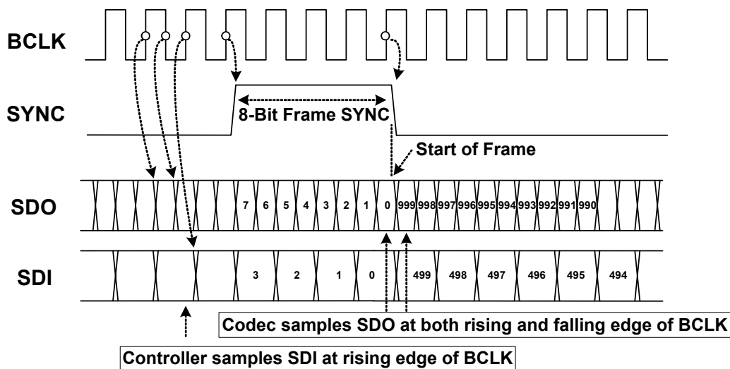
Figure 4. Bit Timing
