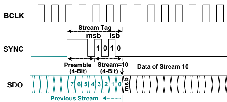
Figure 7. SDO Stream Tag is Indicated in SYNC
