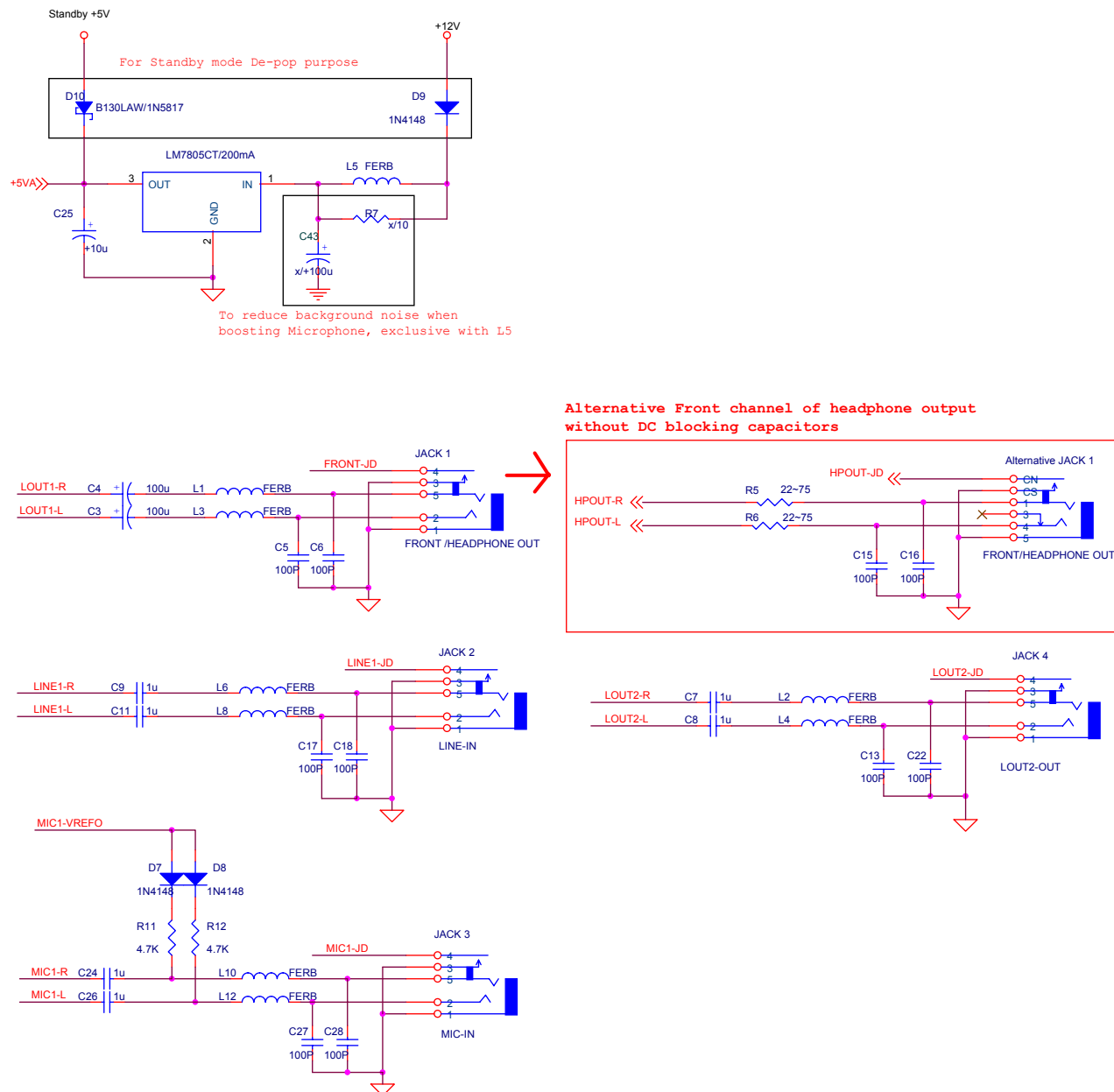
Figure 20. Analog Input/Output Connection
