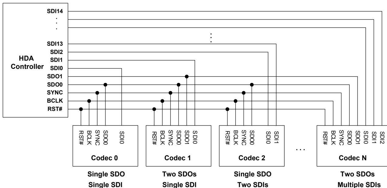
Figure 5. Signaling Topology
