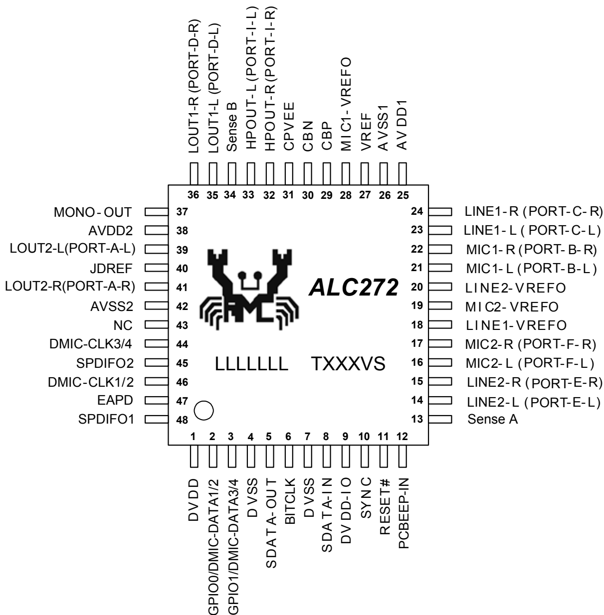
Figure 2. Pin Assignments
