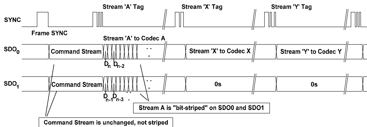
Figure 8. Striped Stream on Multiple SDOs
