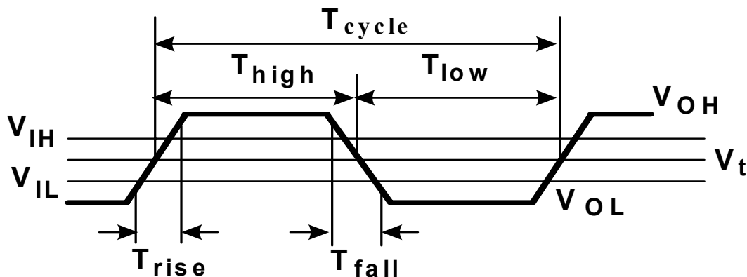
Figure 17. Output Timing
