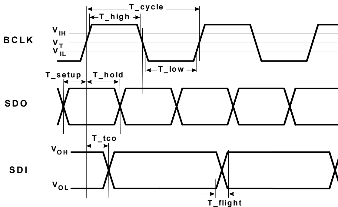
Figure 16. Link Signals Timing
