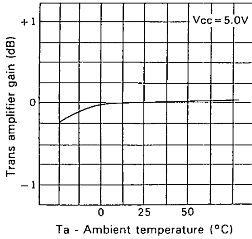
Trans amplifier gain vs. Ambient temperature
