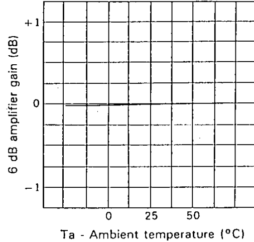
6 dB amplifier gain vs. Ambient temperature
