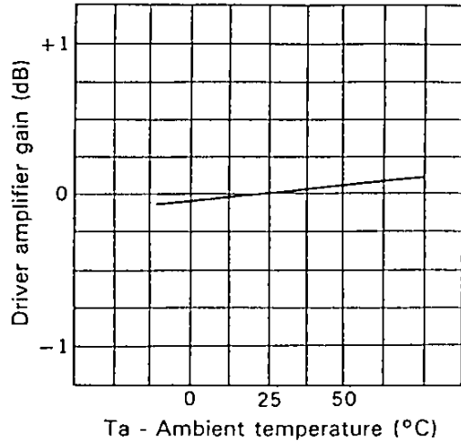
Driver amplifier gain vs. Ambient temperature
