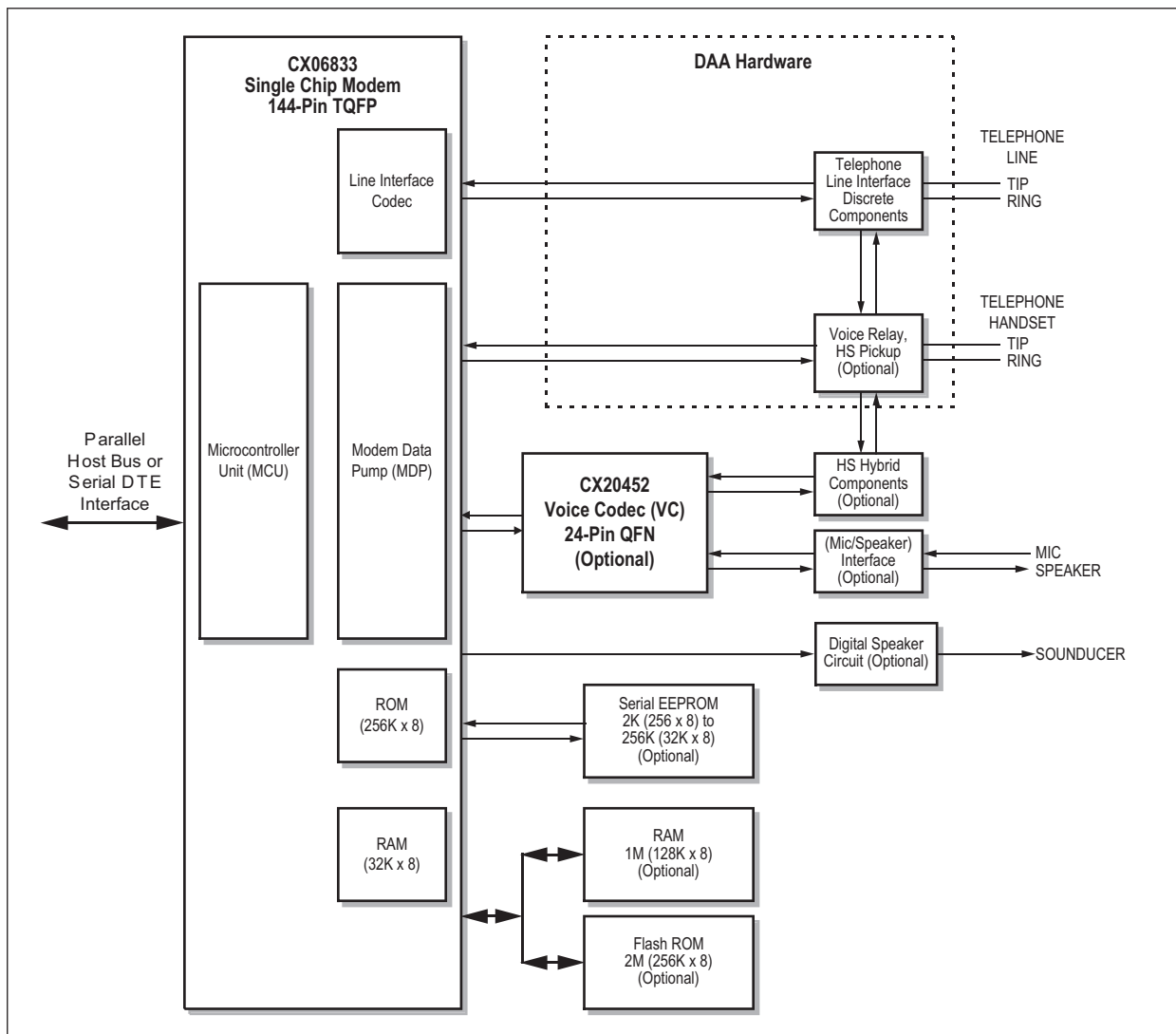
Figure 2. SMXXD Modem Major Interfaces
