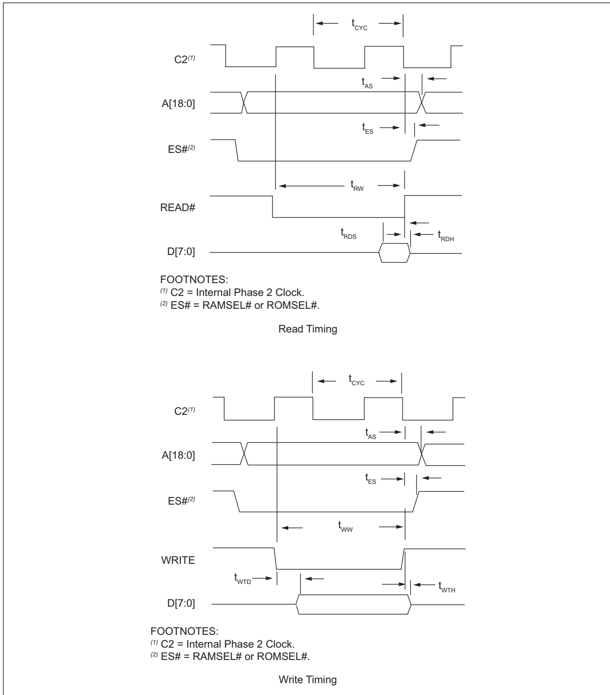
Figure 10. Waveforms - External Memory Bus
