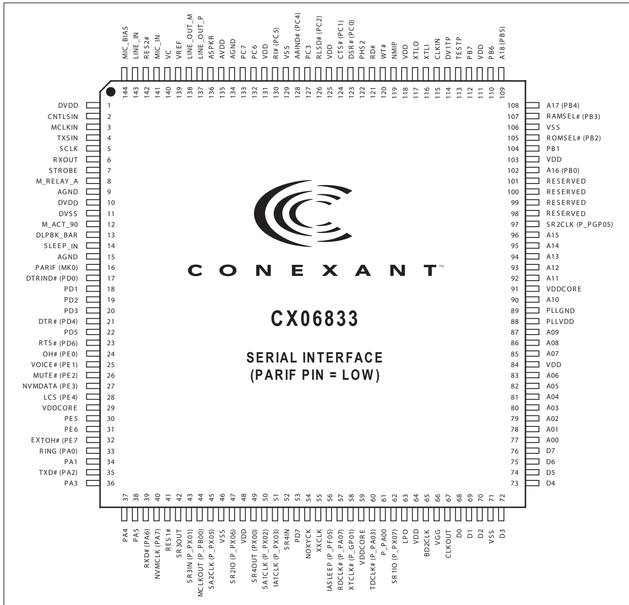
Figure 7. CX06833 144-Pin TQFP Pin Signals for Serial Interface (PARIF = Low)
