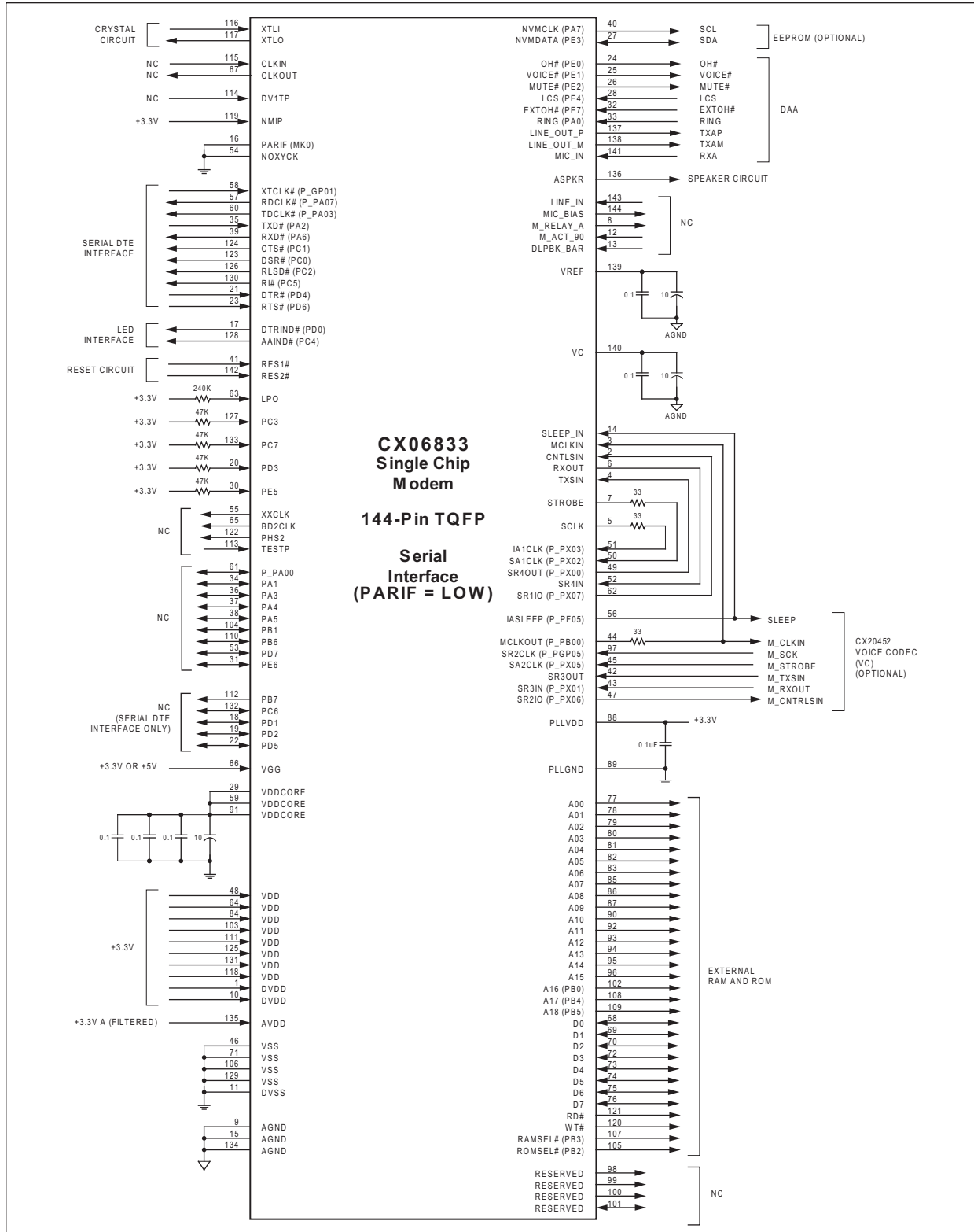
Figure 6. CX06833 Hardware Signals for Serial Interface (PARIF = Low)
