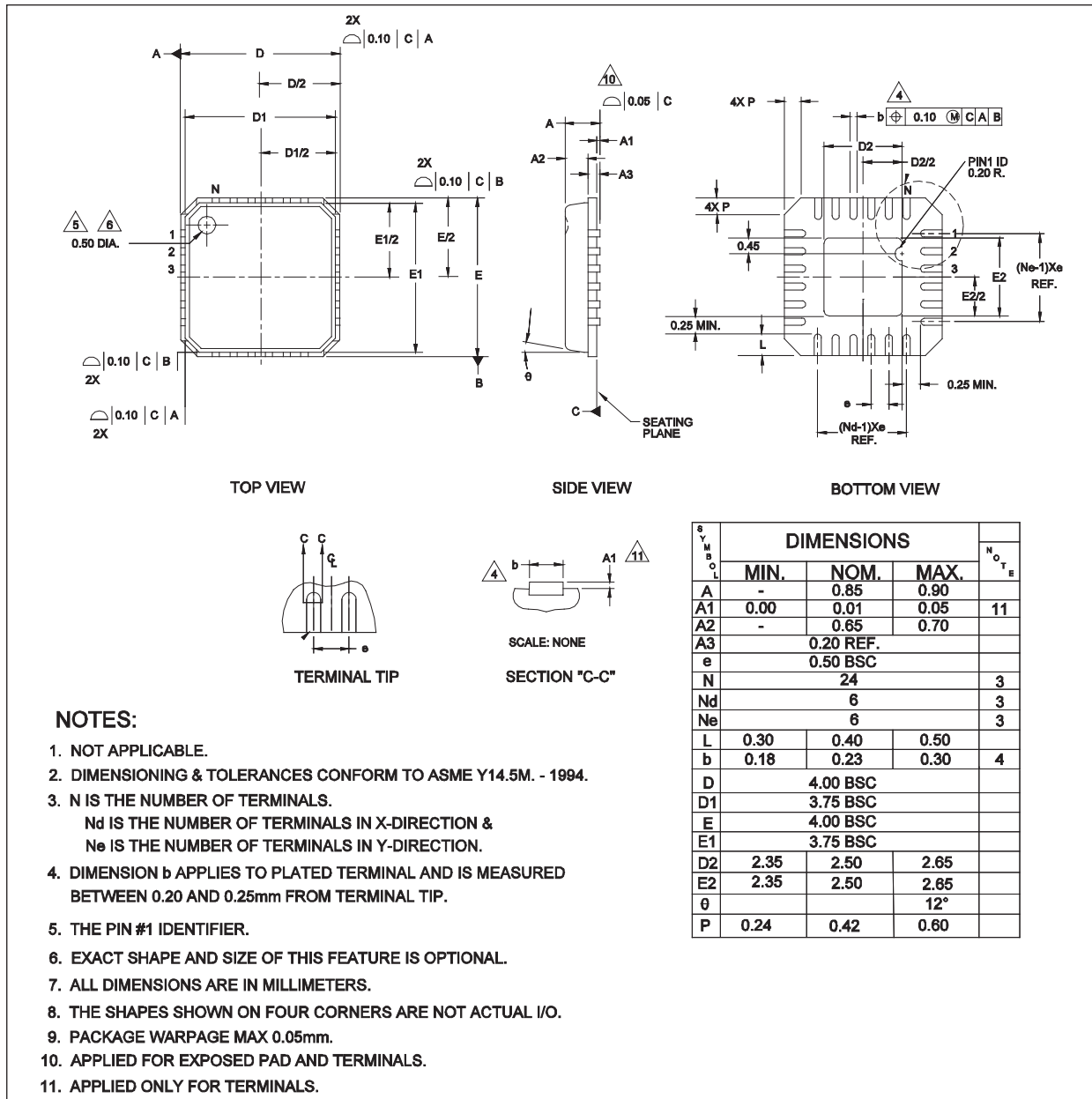
Figure 14. Package Dimensions - 24-Pin QFN
