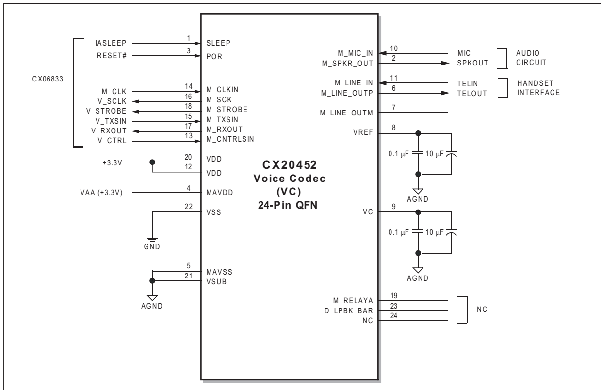
Figure 8. CX20452 VC Hardware Interface Signals
