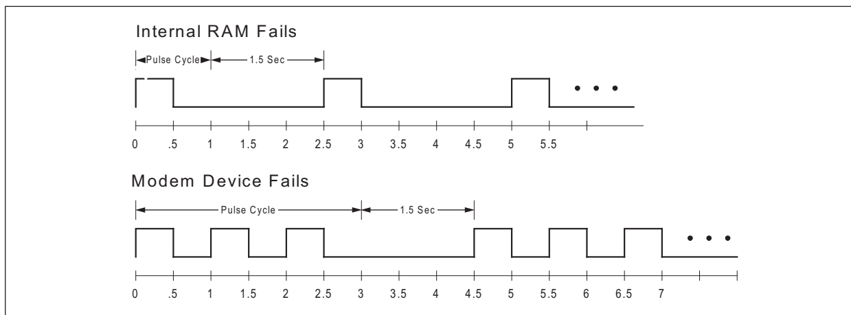
Figure 3. TMIND# Test Results Pulse Cycles
