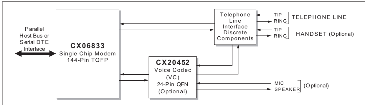
Figure 2. SMXXD Modem Major Interfaces
