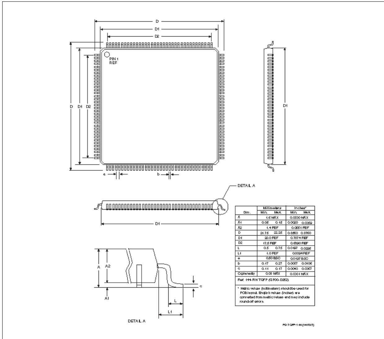
Figure 13. Package Dimensions - 144-Pin TQFP
