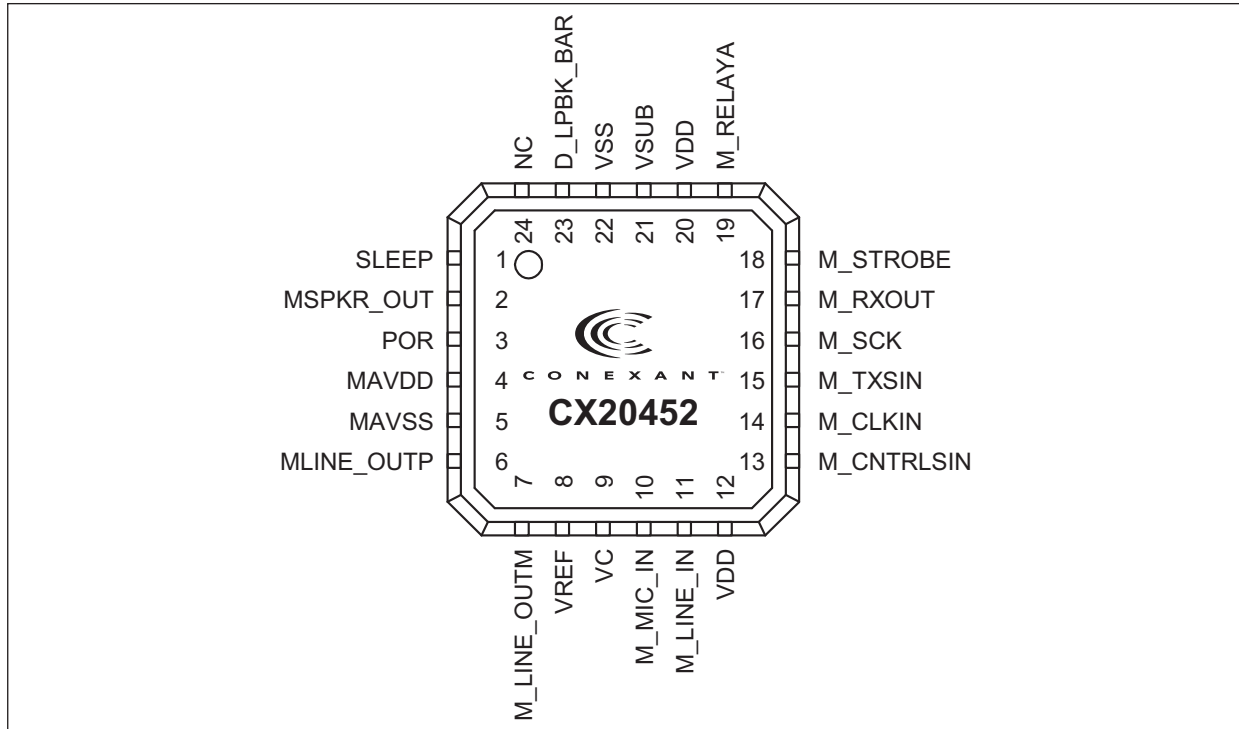
Figure 9. CX20452 VC 24-Pin QFN Pin Signals
