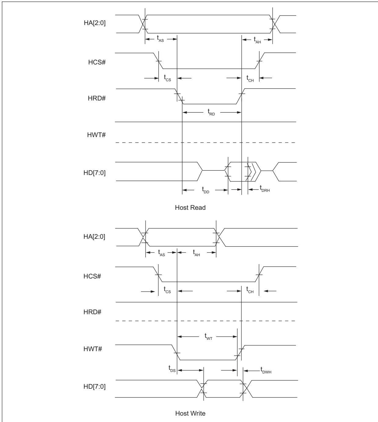
Figure 11. Waveforms - Parallel Host Bus
