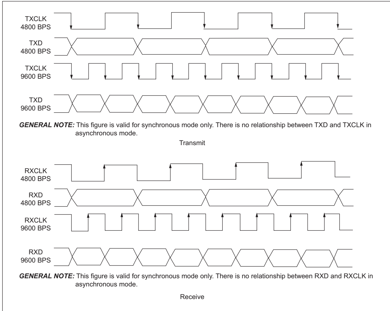
Figure 12. Waveforms - Serial DTE Interface
