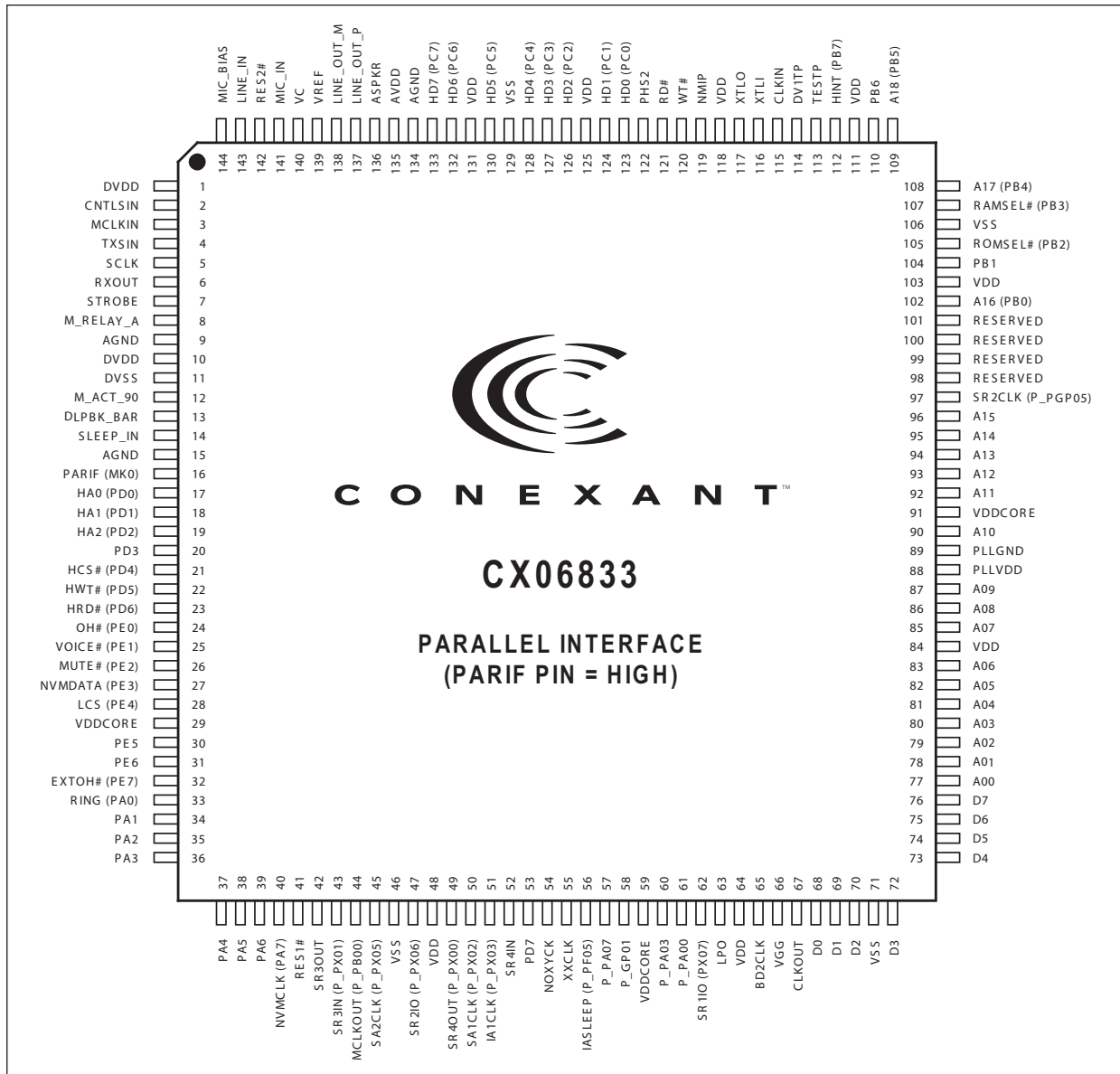
Figure 5. CX06833 144-Pin TQFP Pin Signals for Parallel Interface (PARIF = High)
