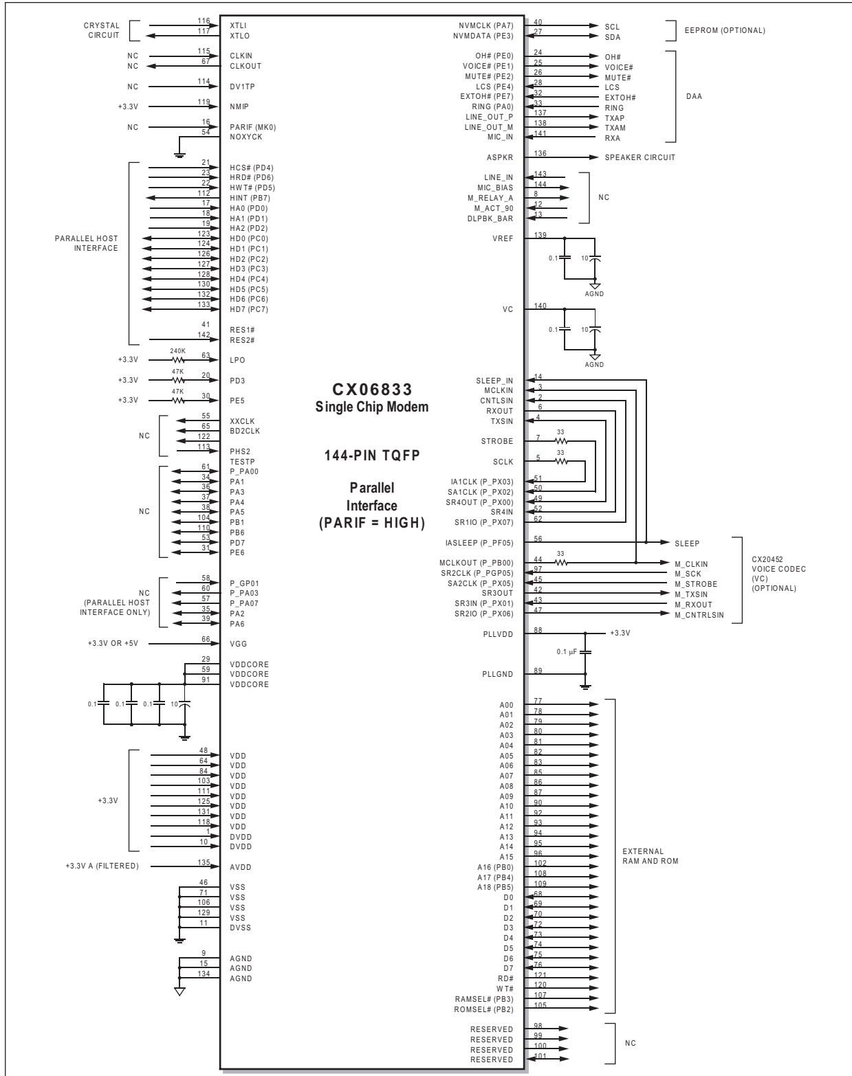
Figure 4. CX06833 Hardware Signals for Parallel Interface (PARIF = High)
