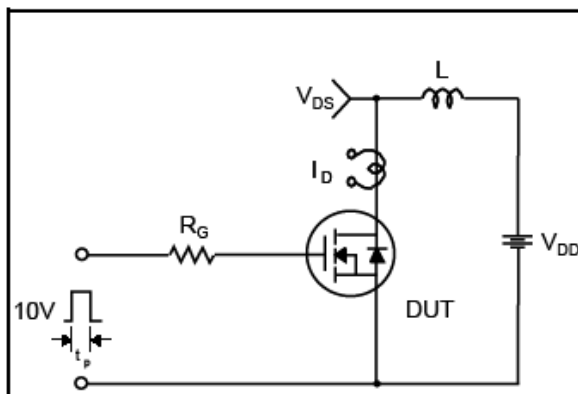
Fig 15. Unclamped Inductive Switching Test Circuit
