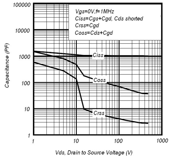
Fig 8. Capacitance Characteristics
