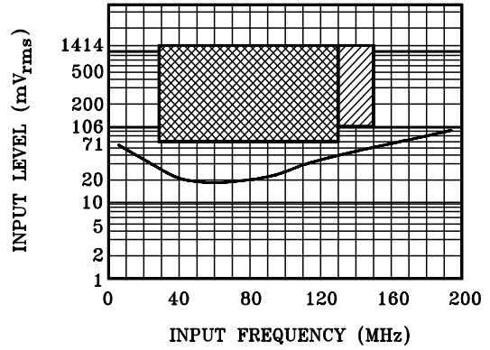
FM IN Frequency Characteristics
