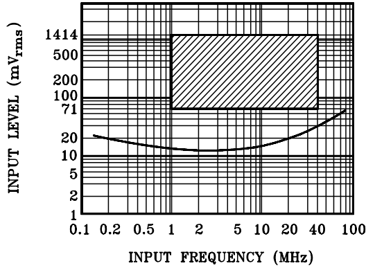
AM IN (HF) Frequency Characteristics
