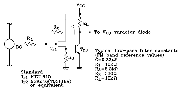
Typical Active Low-Pass Filter Circuit
