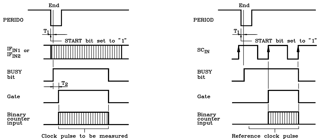
Frequency measurement timing chart
