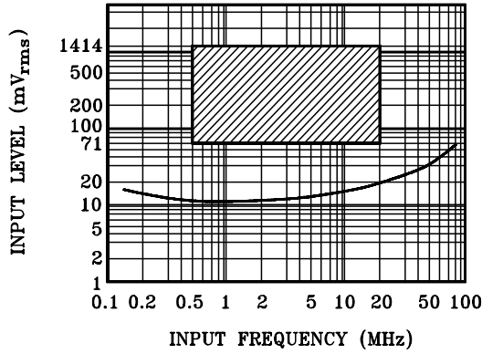
AM IN (LF) Frequency Characteristics
