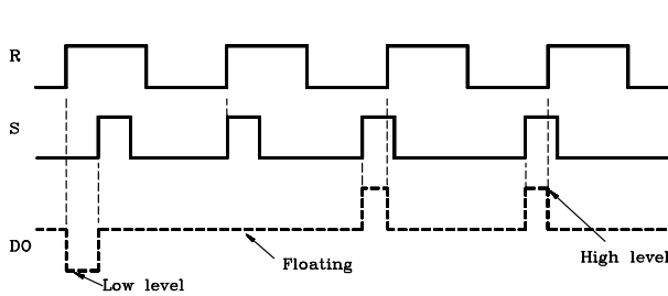
DO Output Timing Chart
