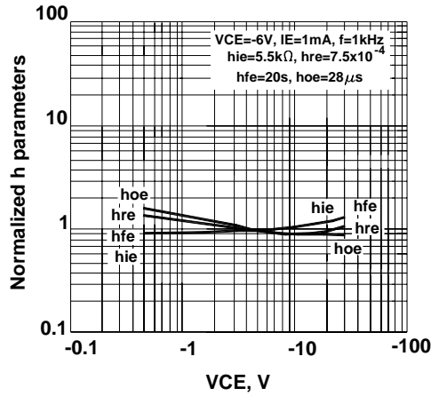
Normalized h-parameters vs. collector emitter voltage
