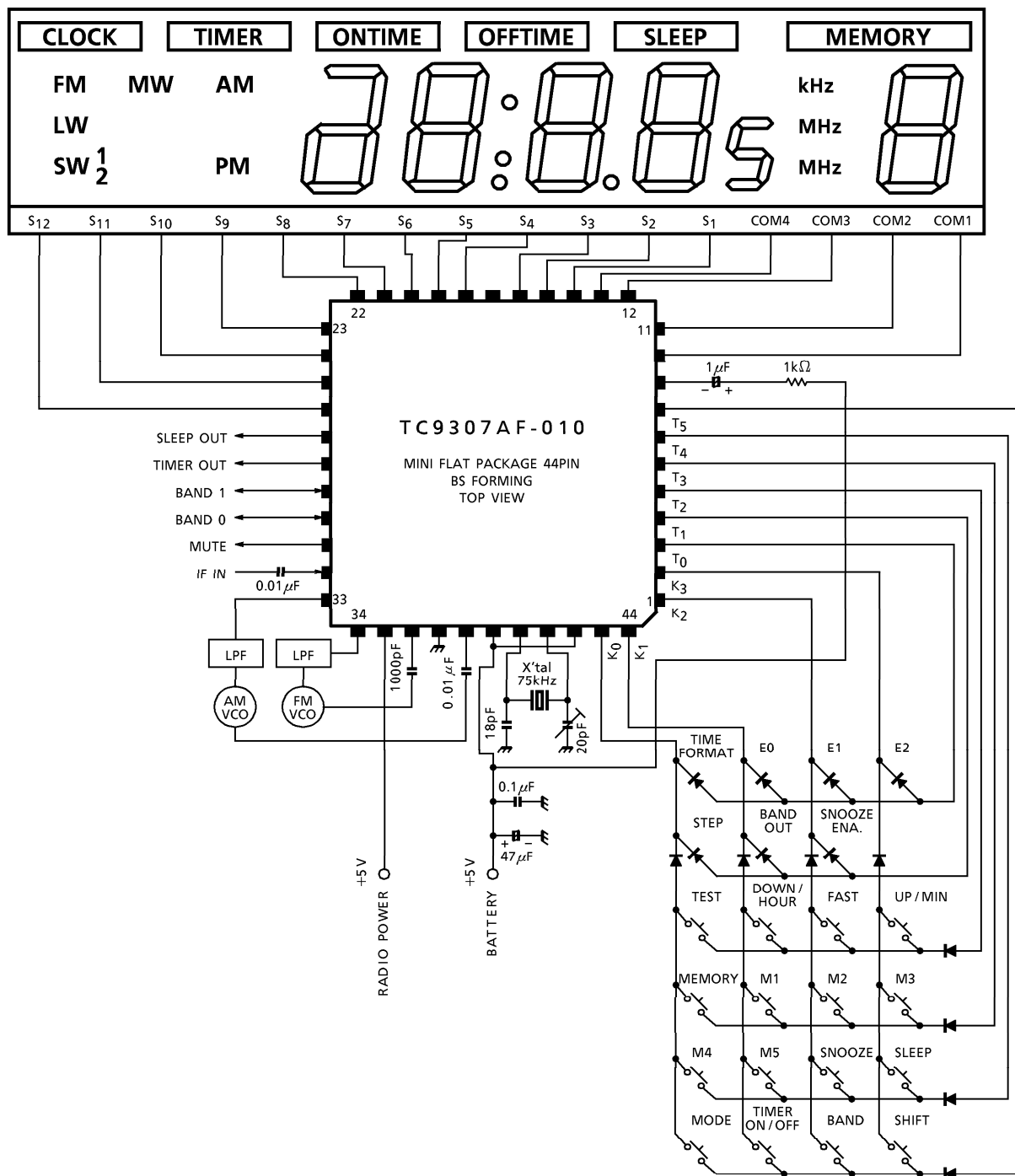
TC9307AF-010 Layout
