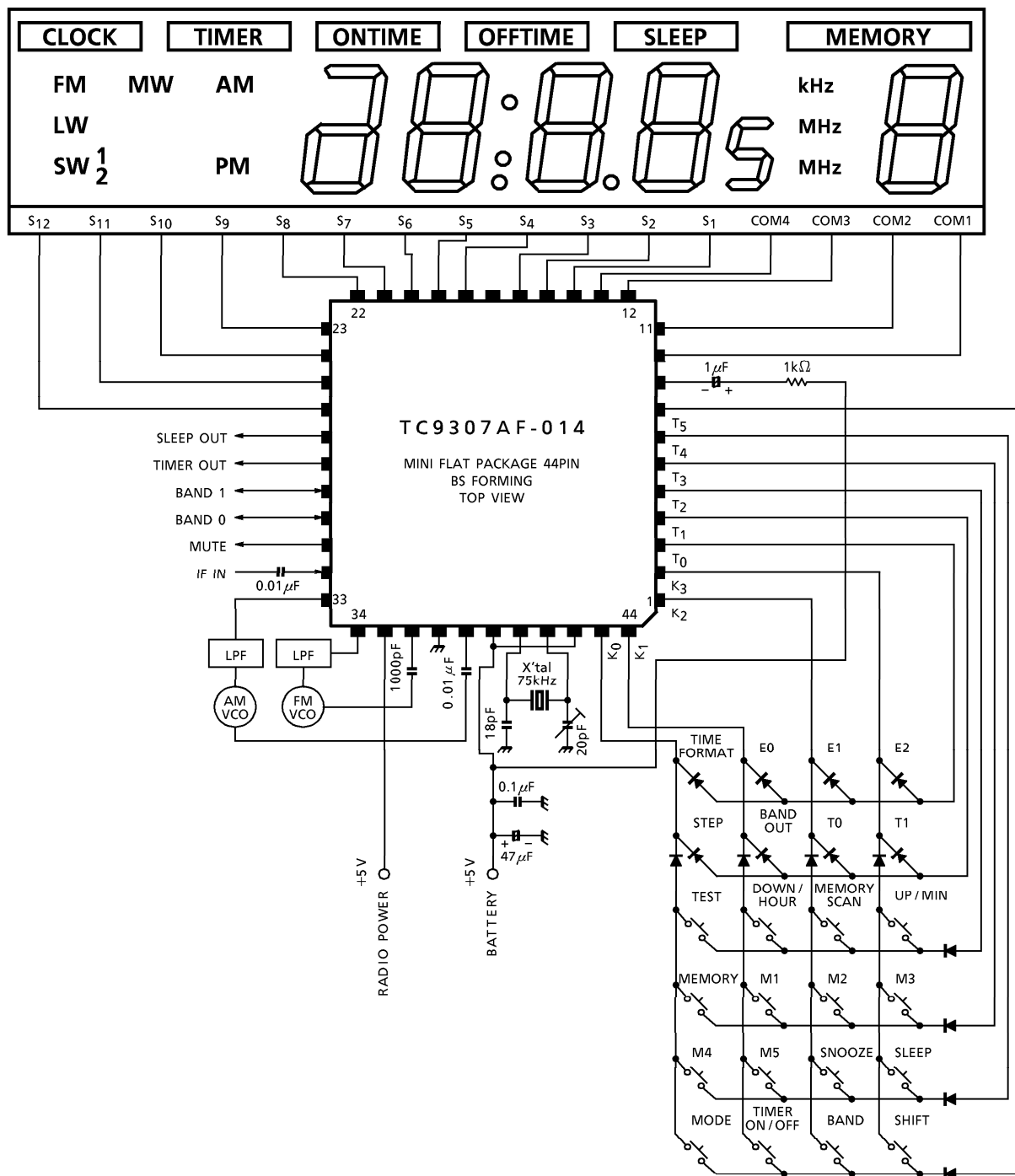
TC9307AF-014 Layout
