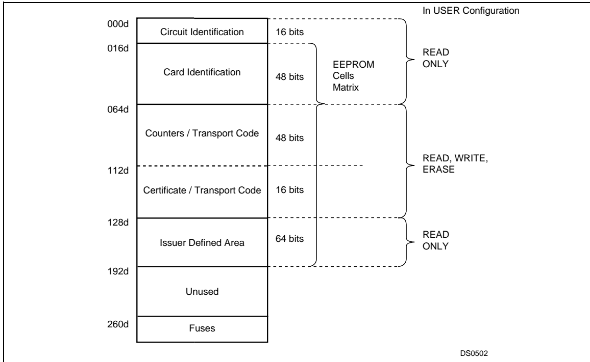
Figure 3. Memory Map
