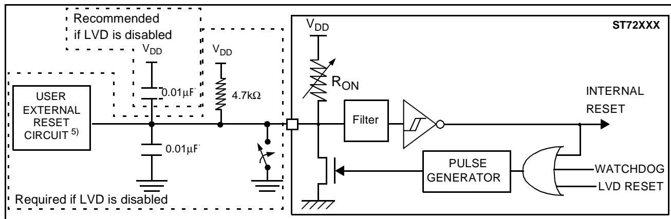
Figure 108. Typical Application with \overline{\text{RESET}} pin 6)7)8)
