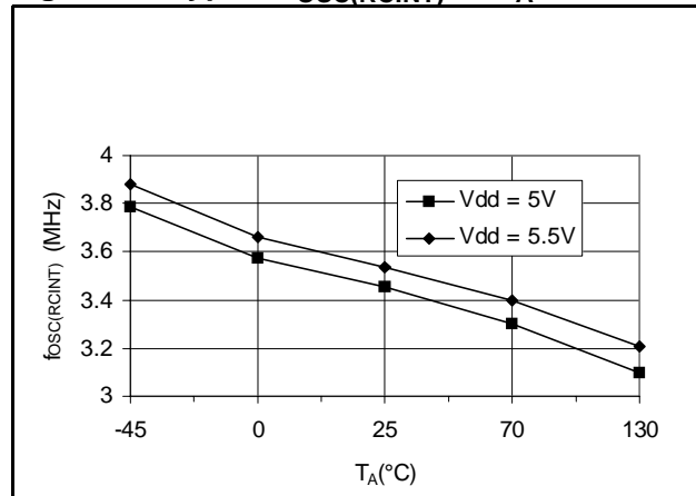
Figure 91. Typical f_{\text{OSC(RCINT)}} vs T_A
