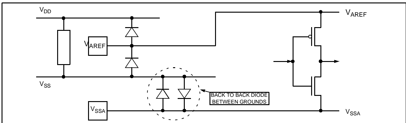
Figure 99. Multisupply Configuration
