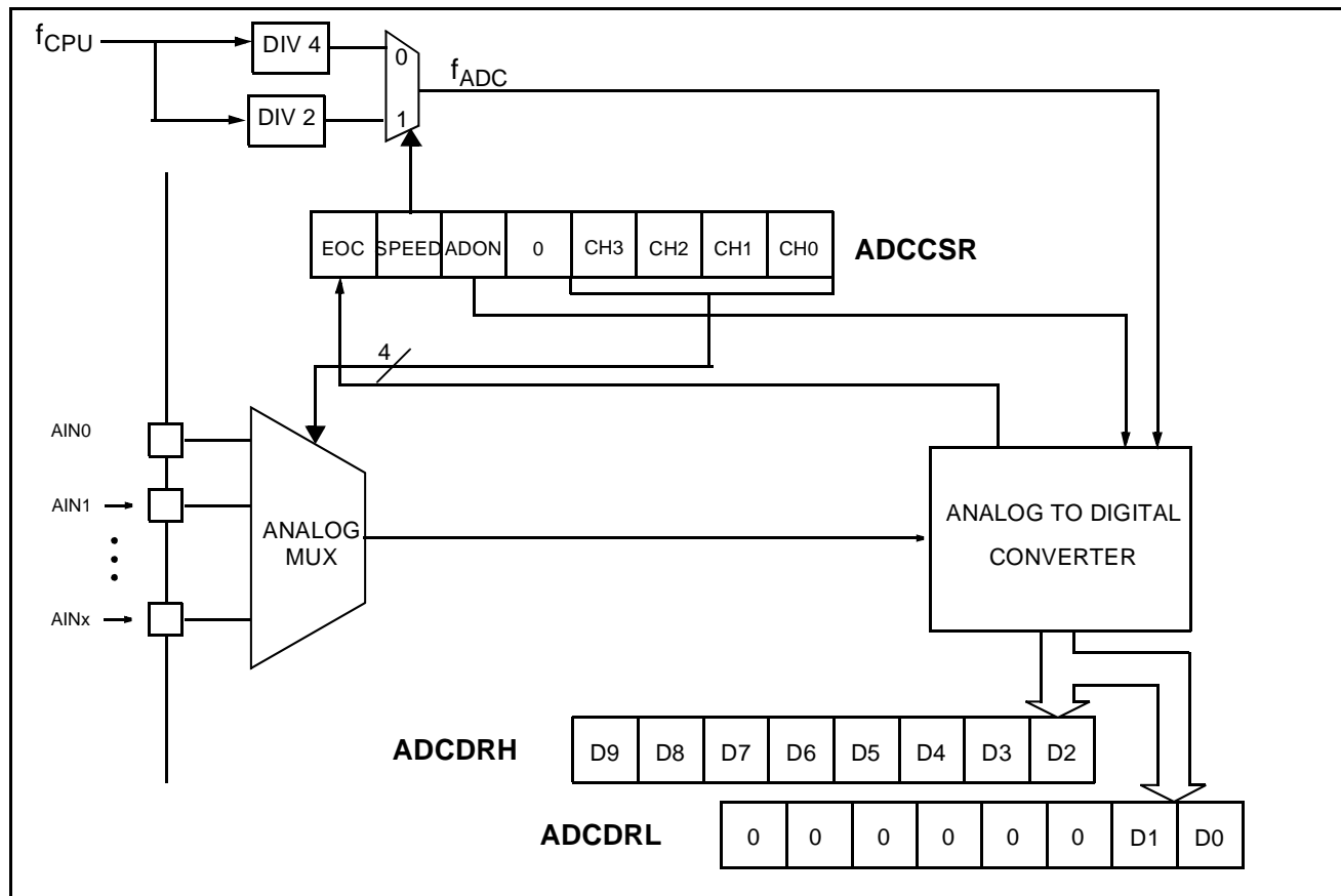
Figure 81. ADC Block Diagram
