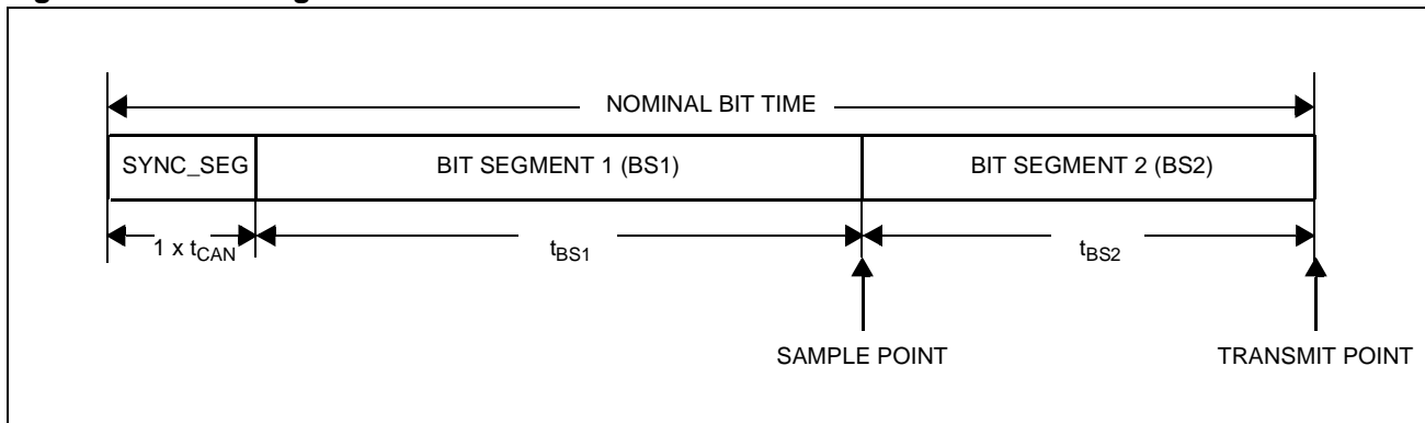
Figure 71. Bit Timing
