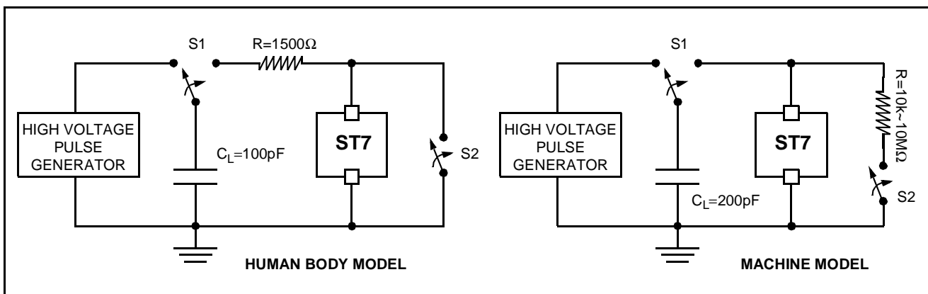
Figure 93. Typical Equivalent ESD Circuits
