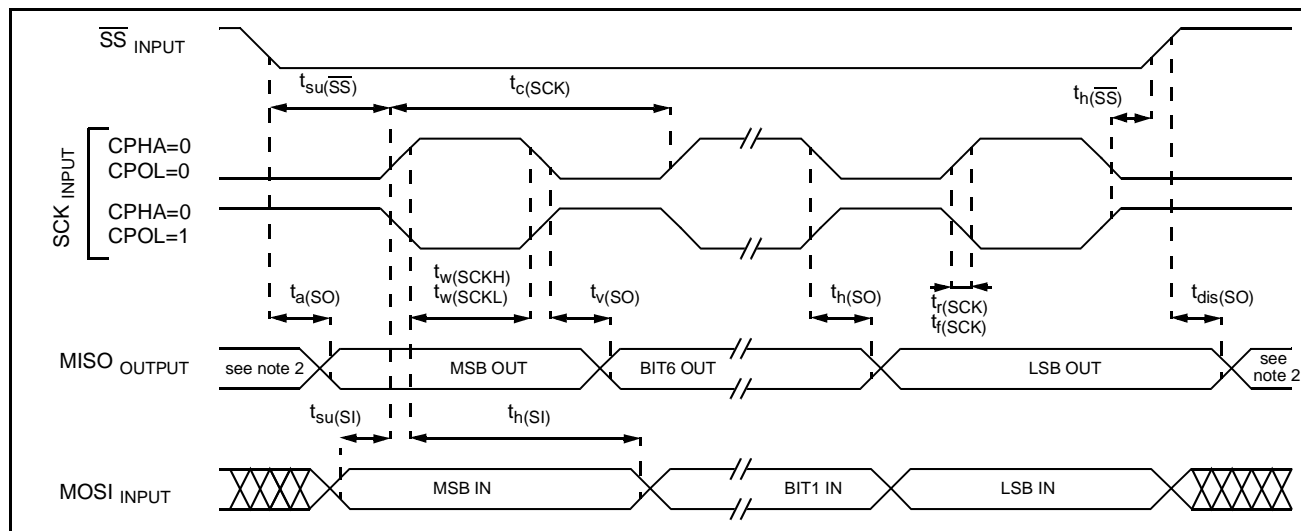
Figure 110. SPI Slave Timing Diagram with CPHA=0 3)
