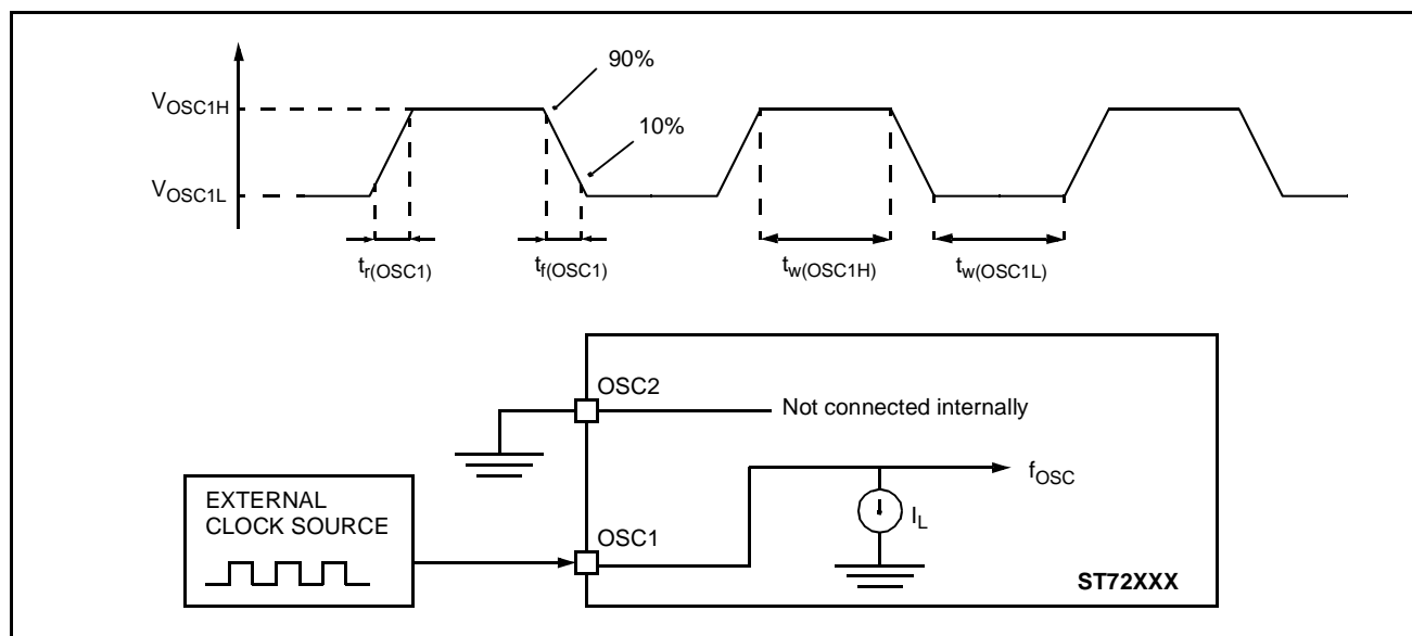
Figure 89. Typical Application with an External Clock Source
