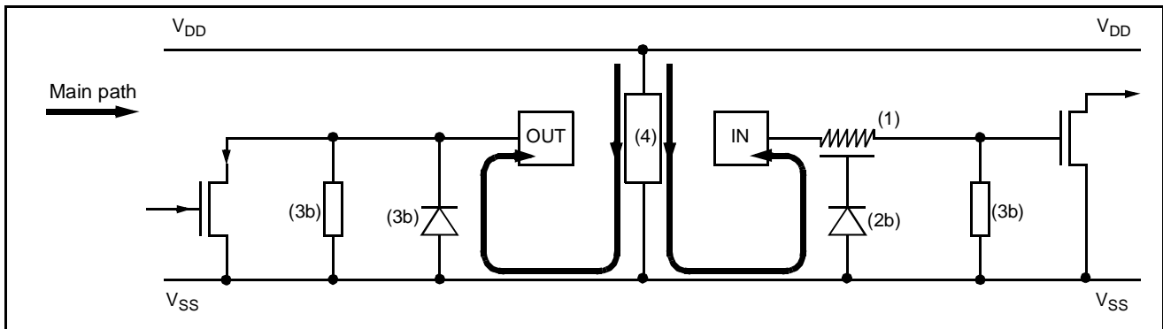
Figure 99. Multisupply Configuration
