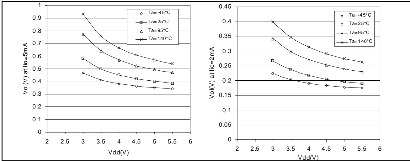
Figure 106. Typical V_{OL} vs. V_{DD} (high-sink)
