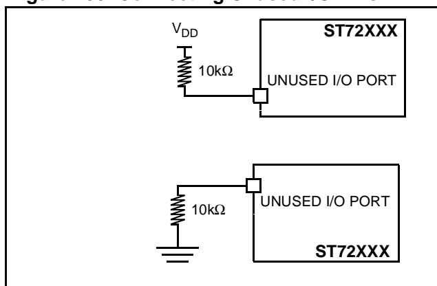
Figure 100. Connecting Unused I/O Pins
