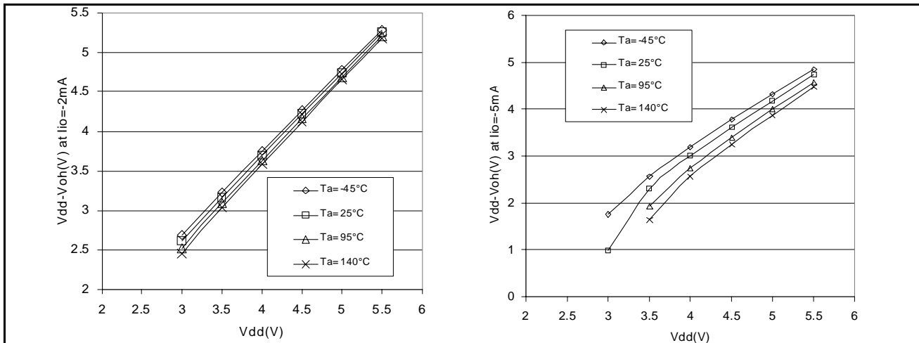
Figure 107. Typical V_{DD} - V_{OH} vs. V_{DD}
