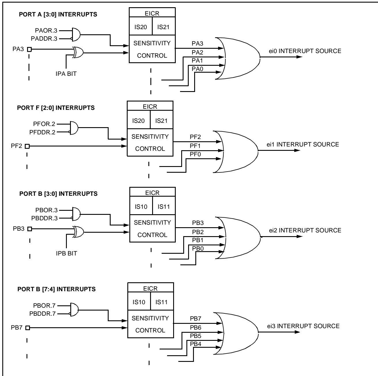
Figure 22. External Interrupt Control bits
