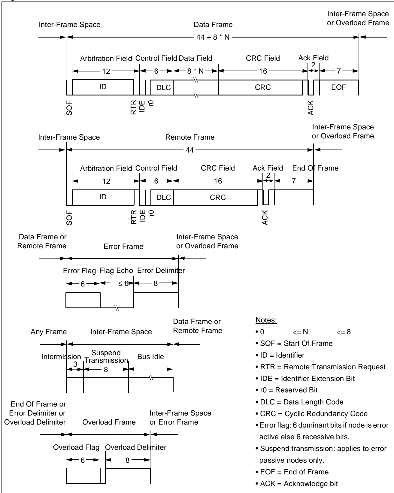
Figure 68. CAN Frames
