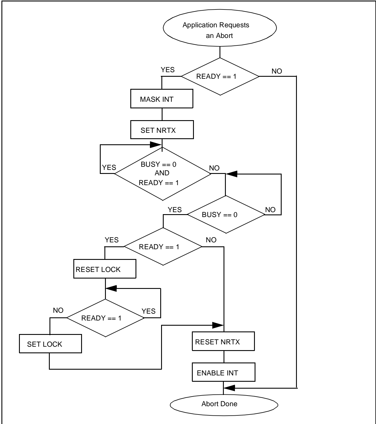
Figure 74. Work-around Flowchart
