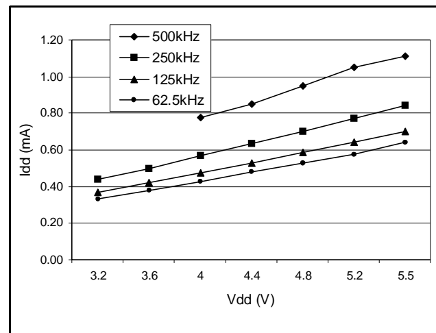
Figure 86. Typical I_{DD} in SLOW vs. f_{CPU}
