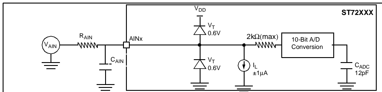
Figure 116. Typical A/D Converter Application
