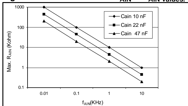
Figure 115. Recommended C_{AIN} & R_{AIN} values. 5)
