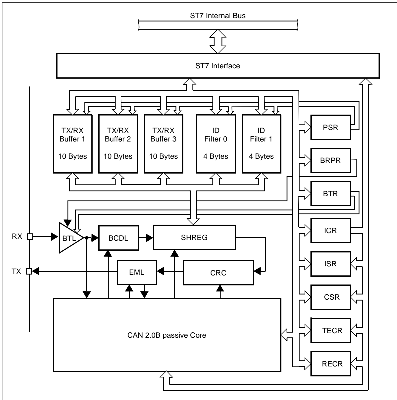
Figure 67. CAN Block Diagram
