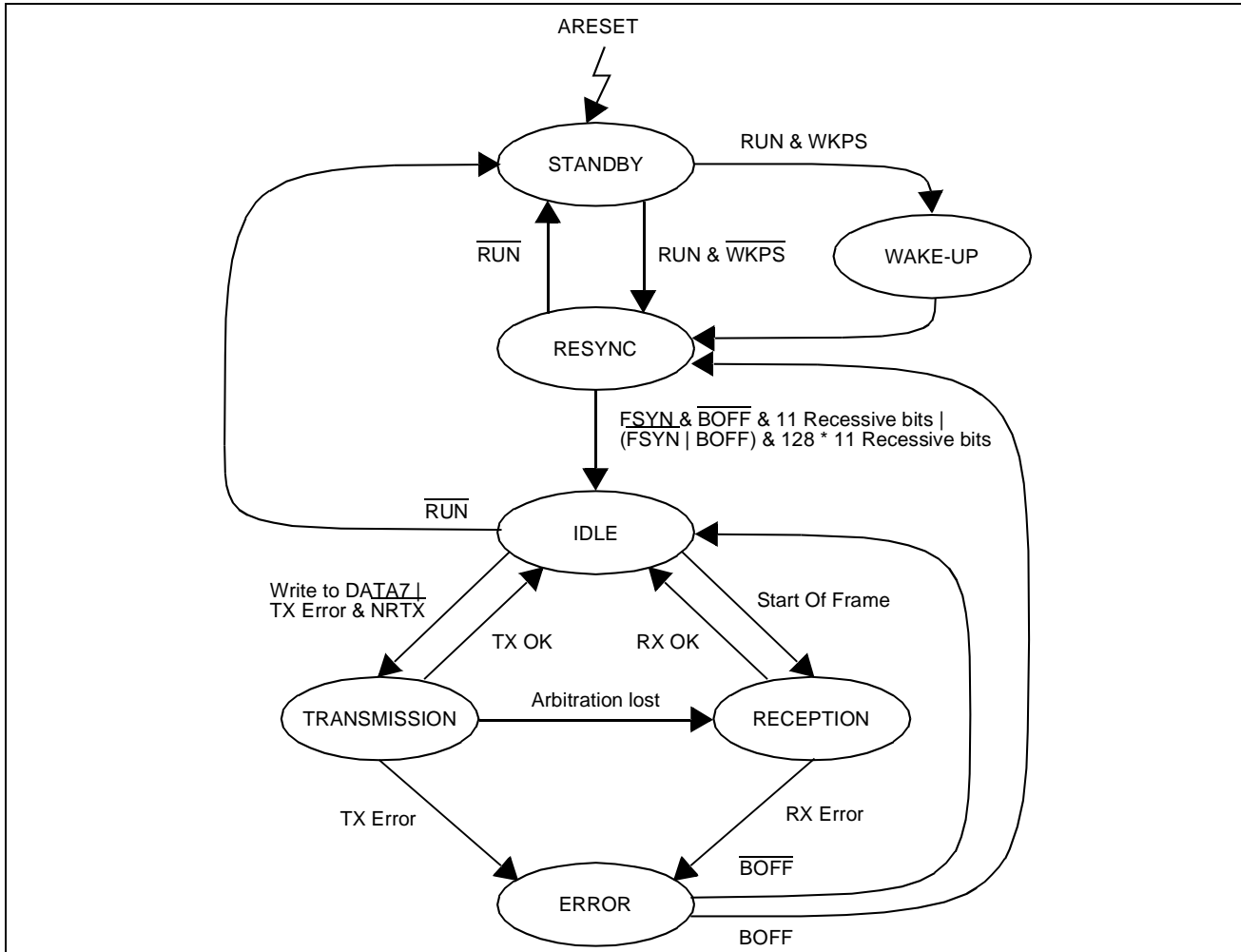
Figure 69. CAN Controller State Diagram
