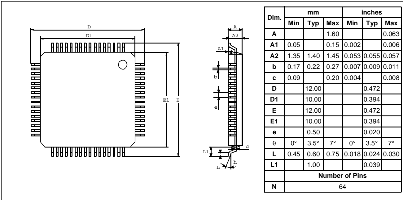
Figure 121. 64-Pin Thin Quad Flat Package
