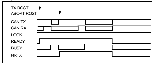
Figure 80. Abort with the software work-around - by NRTX, BUSY and LOCK
