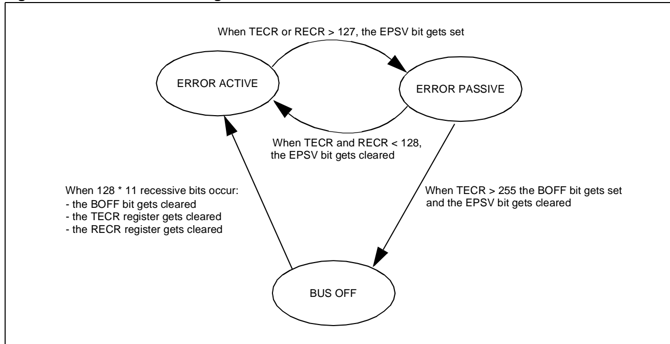
Figure 70. CAN Error State Diagram
