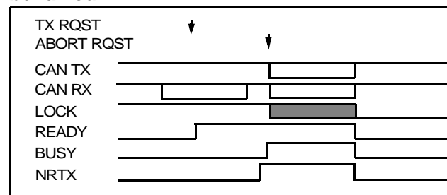
Figure 79. Abort by LOCK only - Reference behaviour
