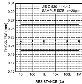
Fig.4 Dimensions (thickness)
