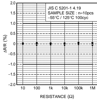
Fig.12 Endurance
