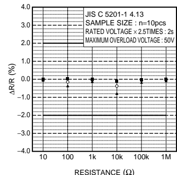
Fig.7 Overload
