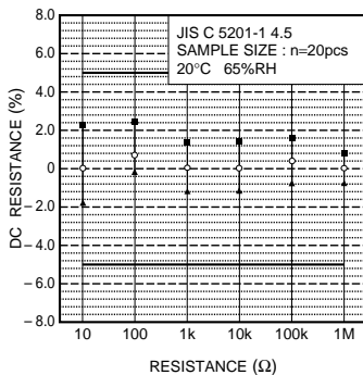
Fig.5 Resistance
