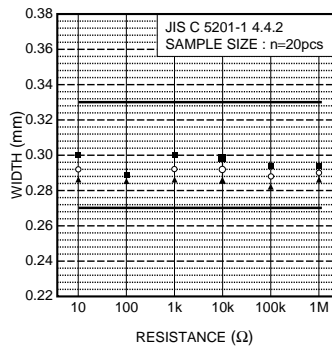
Fig.3 Dimensions (width)
