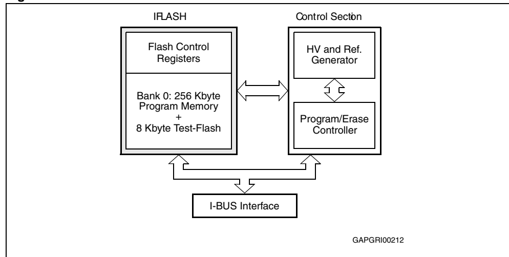
Figure 5. Flash structure
