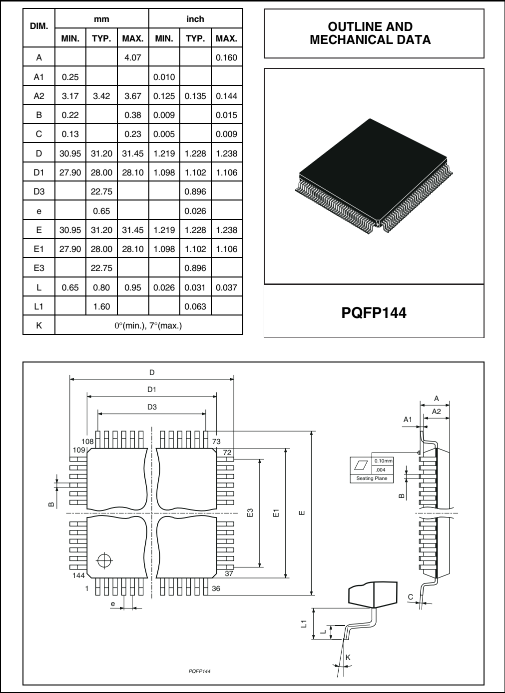
Figure 62. PQFP144 mechanical data and package dimension
