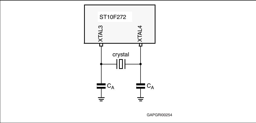
Figure 47. 32kHz crystal oscillator connection diagram
