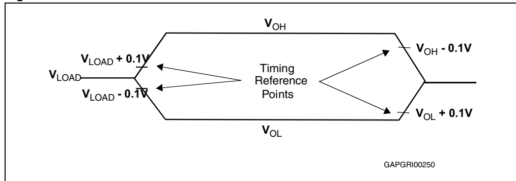
Figure 43. Float waveforms
