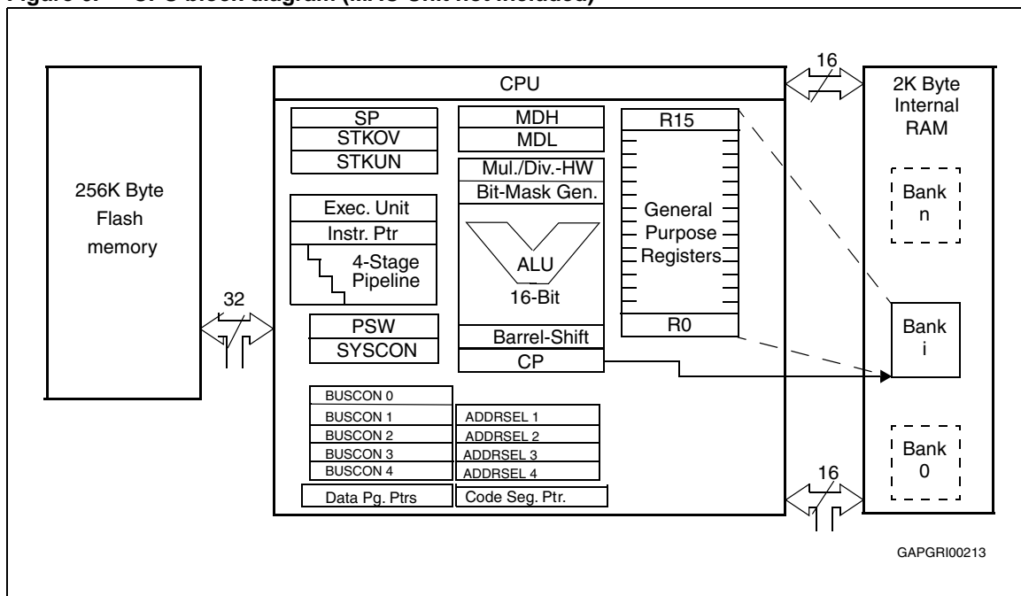
Figure 6. CPU block diagram (MAC Unit not included)
