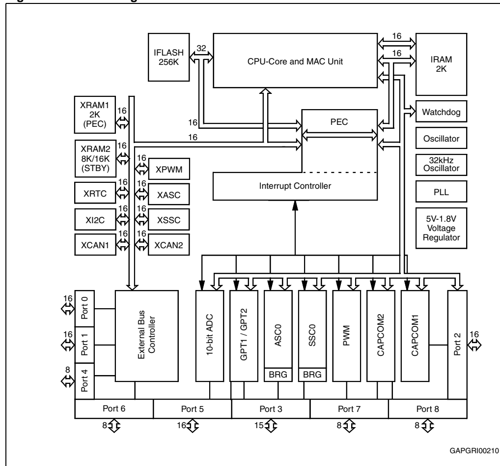
Figure 3. Block diagram
