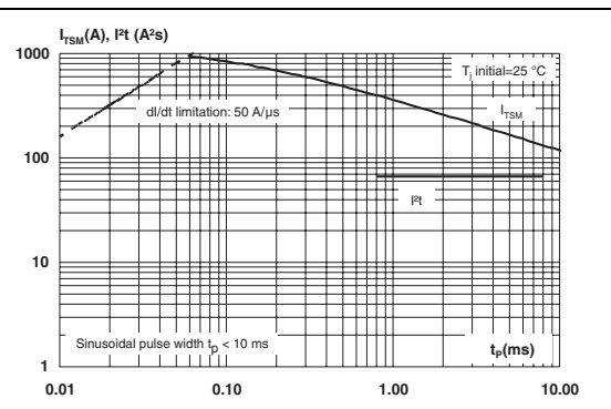
Figure 8. Non-repetitive surge peak on-state current and corresponding value of I^2t
