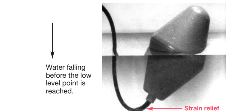
These photographs show the position of the float with rising and falling liquid level.
