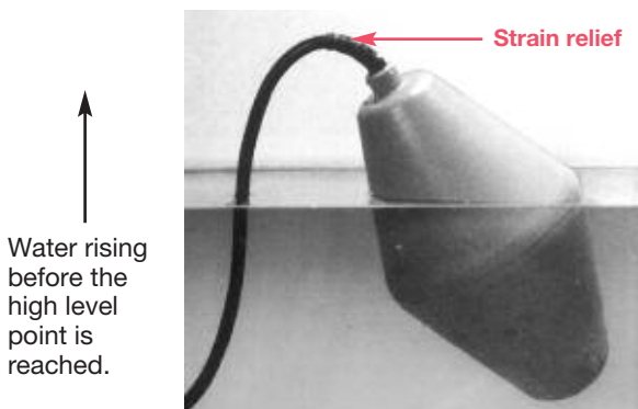
These photographs show the position of the float with rising and falling liquid level.
