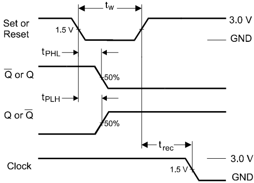
Figure 2. Switching Waveform
