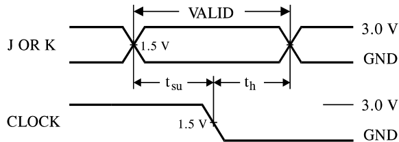
Figure 3. Switching Waveform
