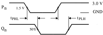
Figure 3. Switching Waveforms
