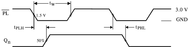
Figure 4. Switching Waveforms
