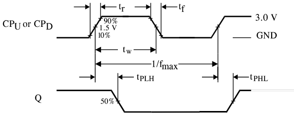
Figure 1. Switching Waveforms
