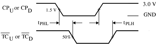
Figure 2. Switching Waveforms
