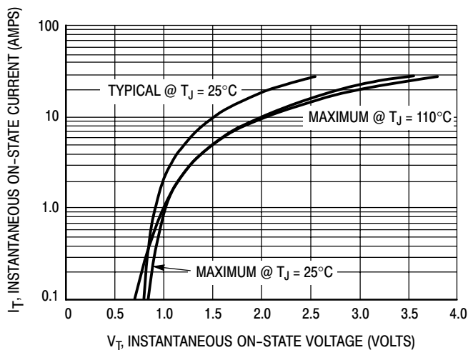
Figure 3. On-State Characteristics
