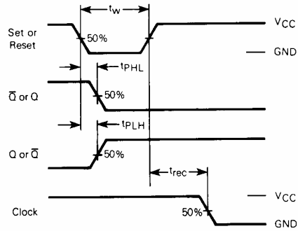
Figure 2. Switching Waveforms
