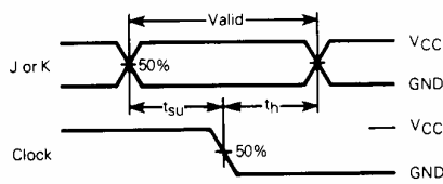
Figure 3. Switching Waveforms
