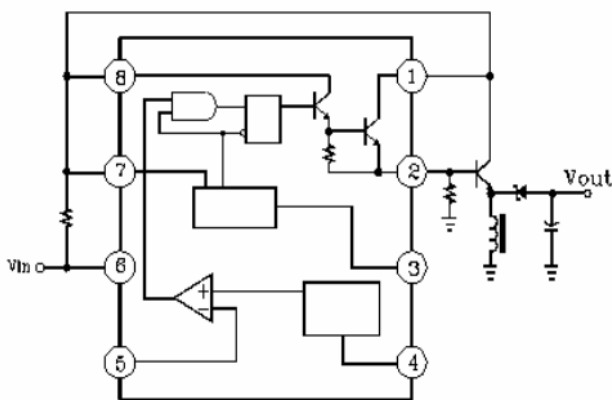
6a.EXTERNAL NPN SWITCH
