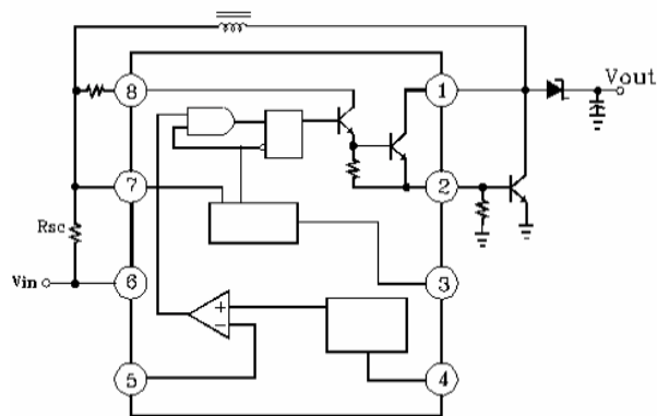
2a.EXTERNAL NPN SWITCH
