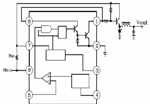
4b.EXTERNAL NPN SWITCH
