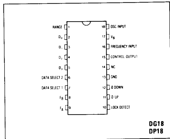
Fig.1 Pin connections
