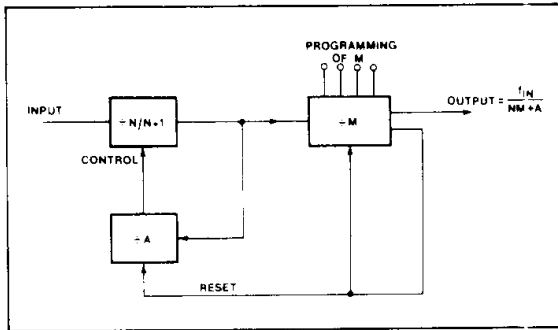
Fig.5 2-modulus counter
