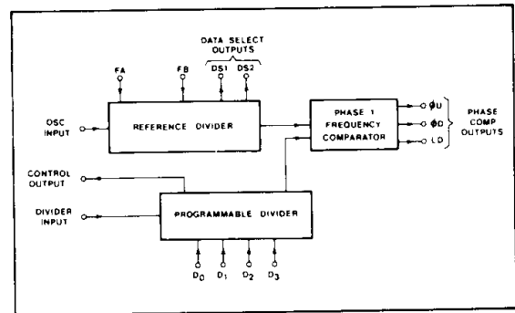
Fig.2 NJ8812 Block diagram
