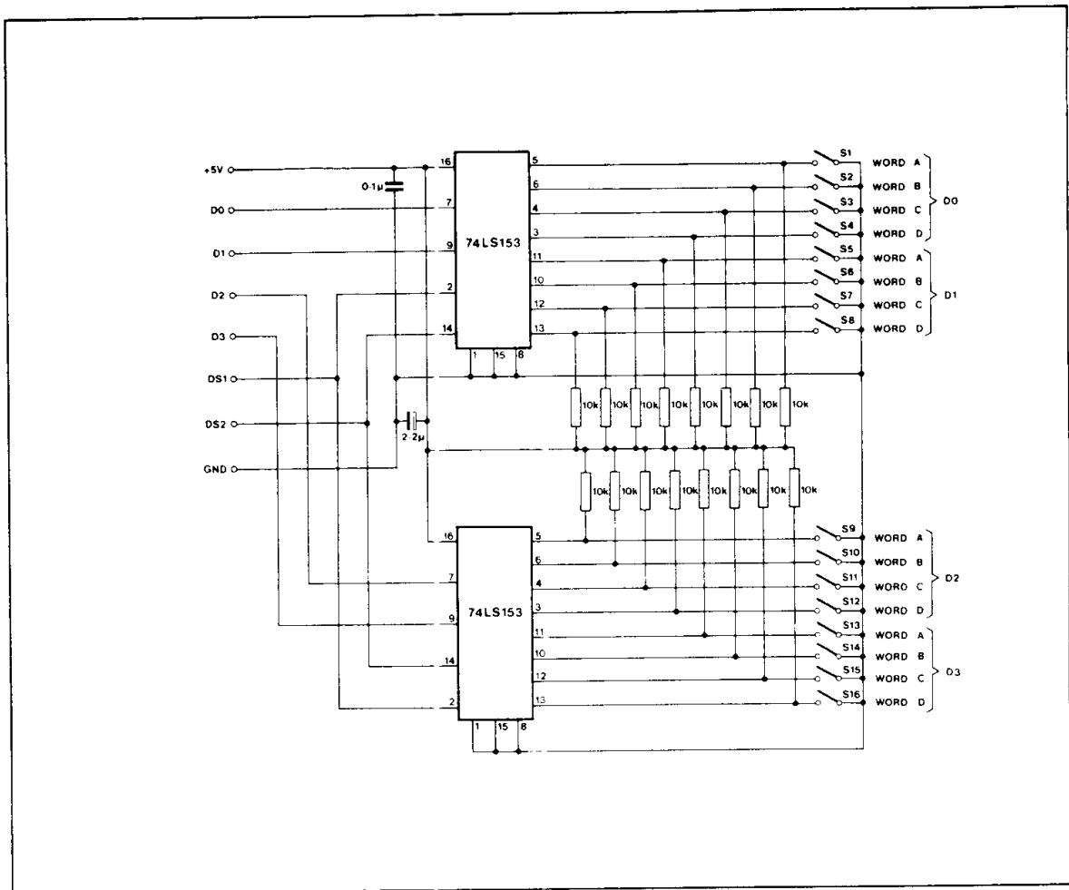
Fig 8 Programming board
