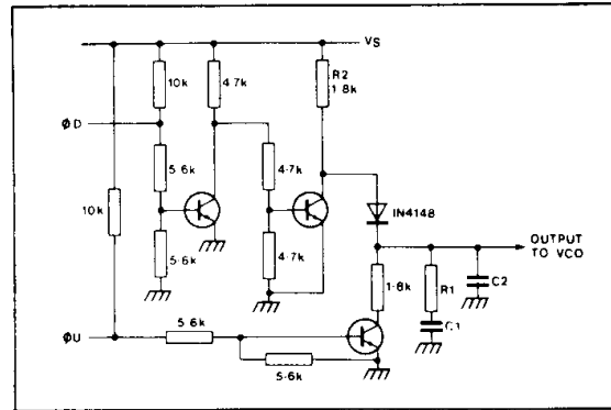
Fig.7 Circuit for combining \Phi_D and \Phi_U
