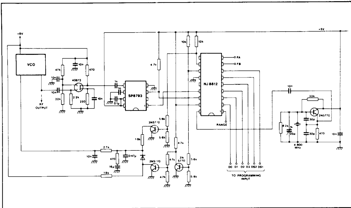
Fig 9 Frequency synthesiser using NJ8812 and SP8793
