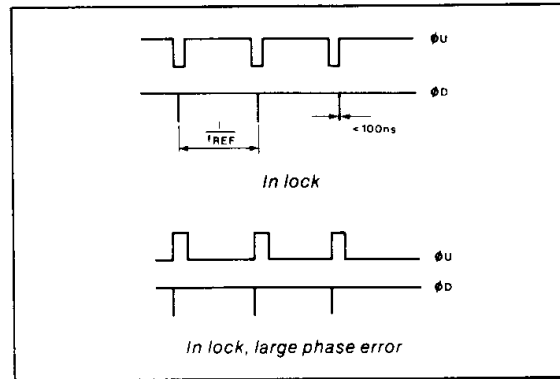
Fig.6 Phase detector waveforms
