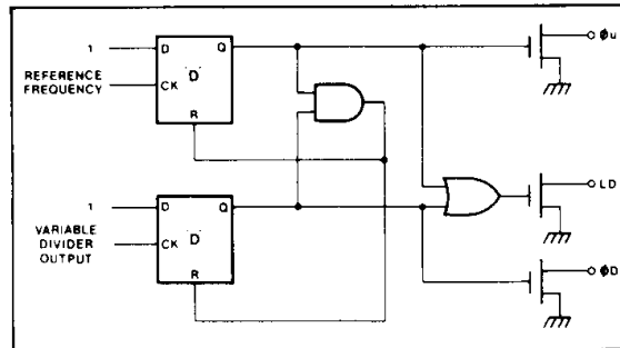
Fig.3 Logic diagram
