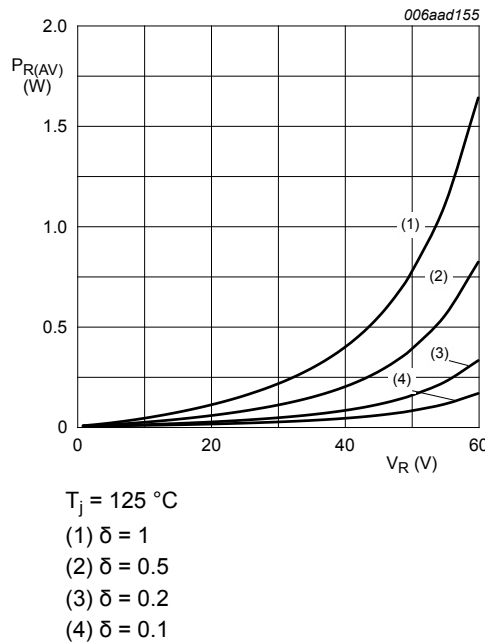
Fig. 9. Average reverse power dissipation as a function of reverse voltage; typical values T_j = 125\text{ °C} (1) \delta = 1 (2) \delta = 0.5 (3) \delta = 0.2 (4) \delta = 0.1
