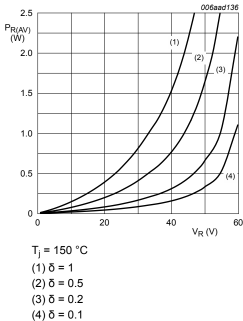
Fig. 8. Average reverse power dissipation as a function of reverse voltage; typical values T_j = 150\text{ °C} (1) \delta = 1 (2) \delta = 0.5 (3) \delta = 0.2 (4) \delta = 0.1
