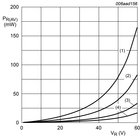
T_j = 85\text{ }^\circ\text{C} (1) \delta = 1 (2) \delta = 0.5 (3) \delta = 0.2 (4) \delta = 0.1
