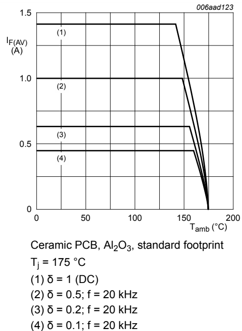
Fig. 13. Average forward current as a function of ambient temperature; typical values
