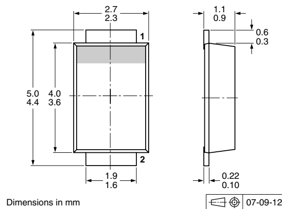
Fig 14. Package outline SOD128
