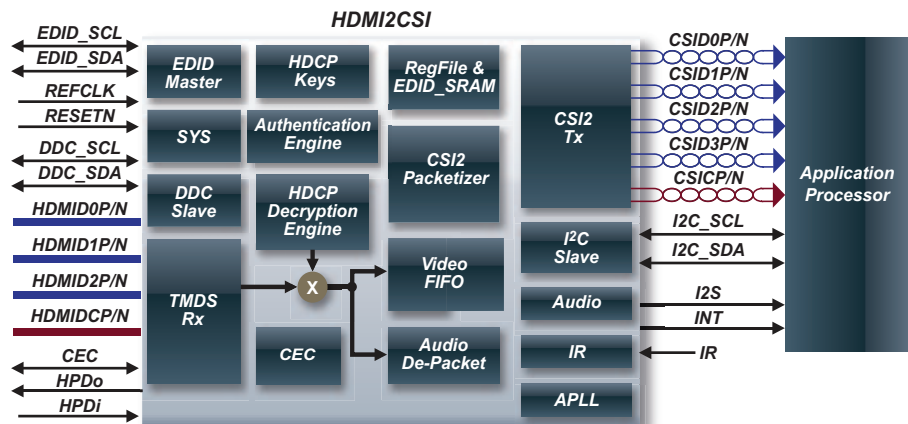
TC358743XBG Block Diagram: HDMI to CSI-2 Bridge Chip
