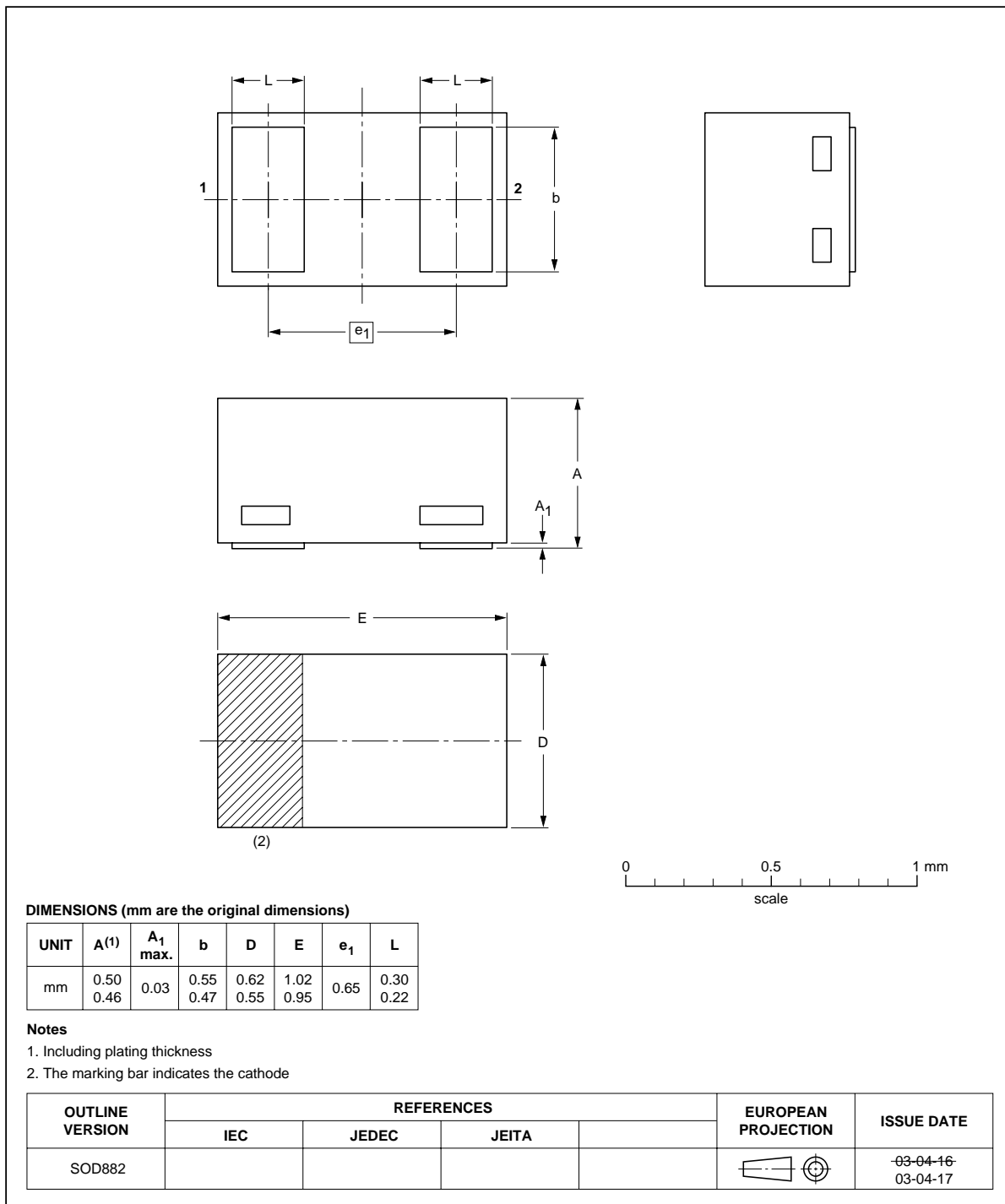
Fig 4. Package outline.
