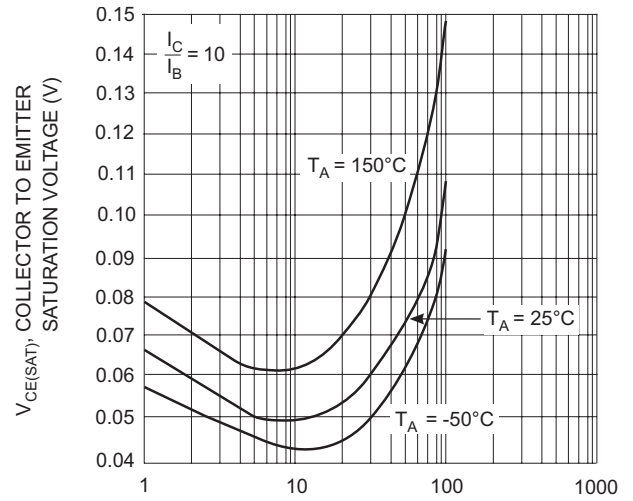
I_C , COLLECTOR CURRENT (mA) Fig. 2, Collector Emitter Saturation Voltage vs. Collector Current (NPN5551)
