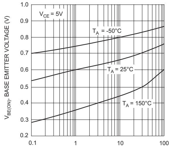
I_C , COLLECTOR CURRENT (mA) Fig. 4, Base Emitter Voltage vs. Collector Current (NPN5551)
