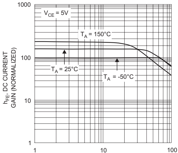
I_C , COLLECTOR CURRENT (mA) Fig. 3, DC Current Gain vs Collector Current (NPN5551)
