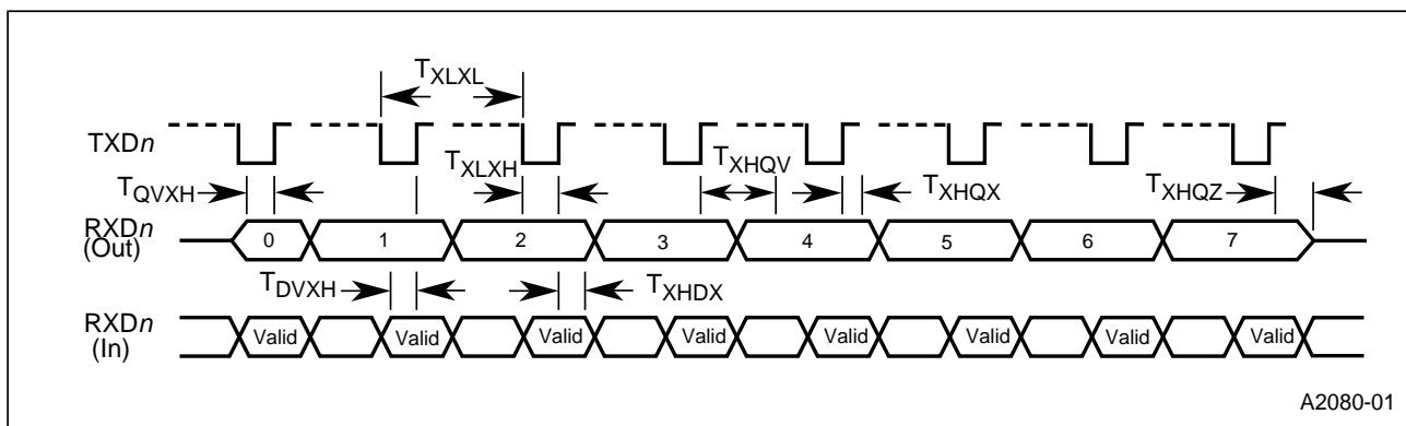
Figure 15. Serial Port Waveform — Shift Register Mode (Mode 0)
