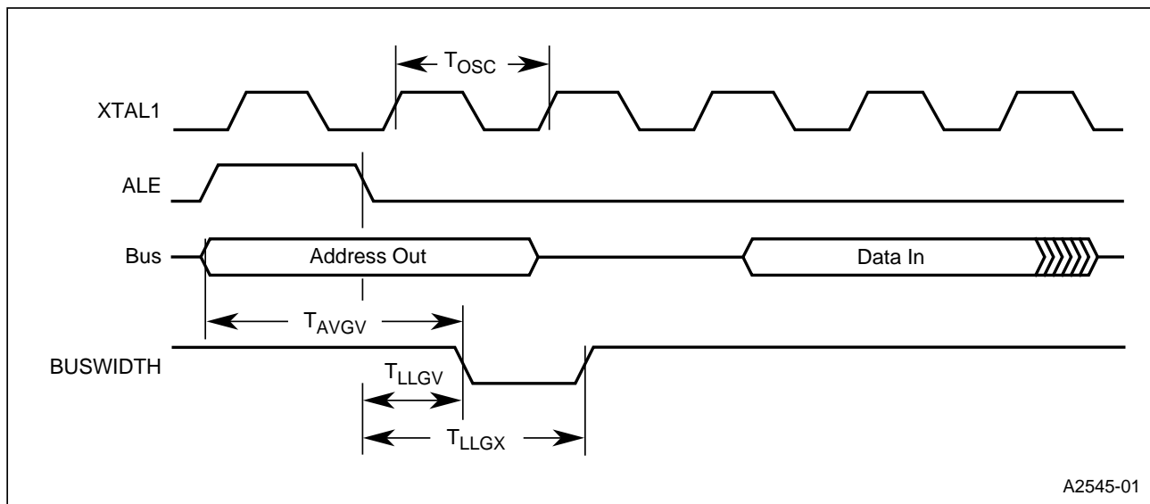
Figure 9. BUSWIDTH Timing Diagram
