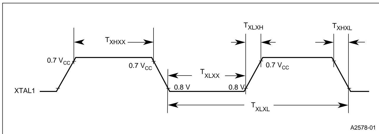
Figure 10. External Clock Drive Waveforms
