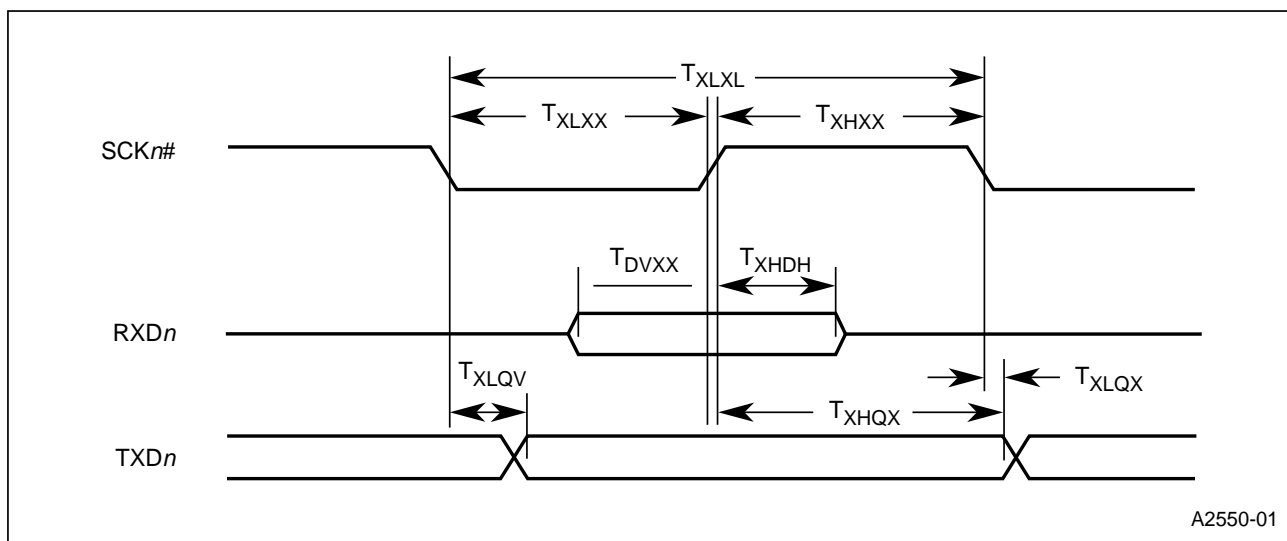
Figure 16. Serial Port Waveform — Mode 4
