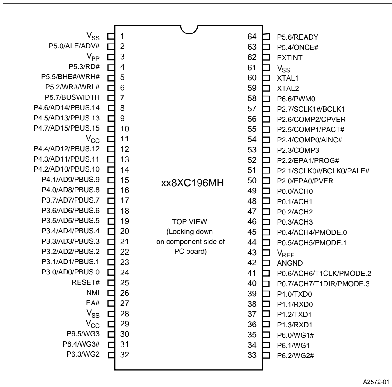
Figure 3. 8XC196MH 64-lead Shrink DIP (SDIP) Package
