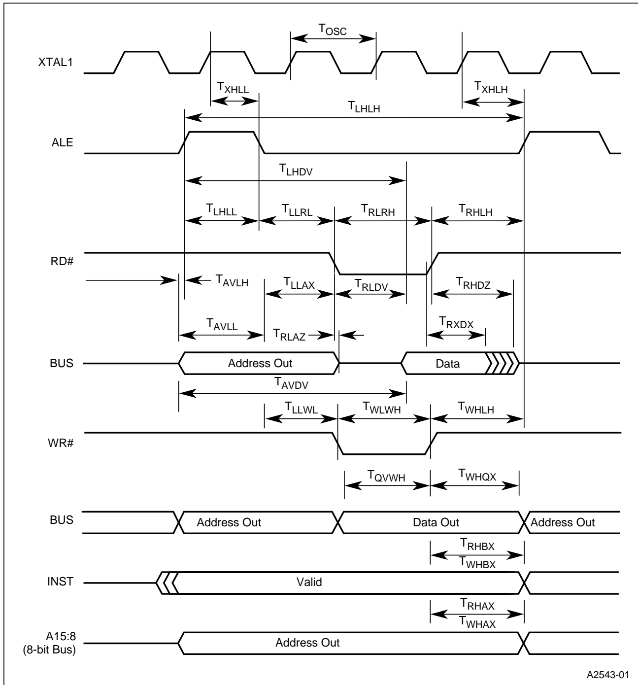
Figure 7. System Bus Timing Diagram
