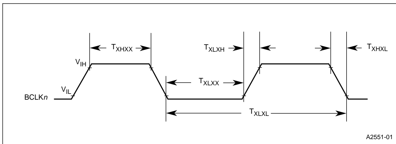
Figure 18. Baud-Rate Clock Drive Waveforms
