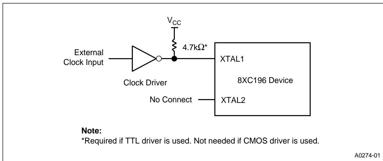
Figure 11. External Clock Connections
