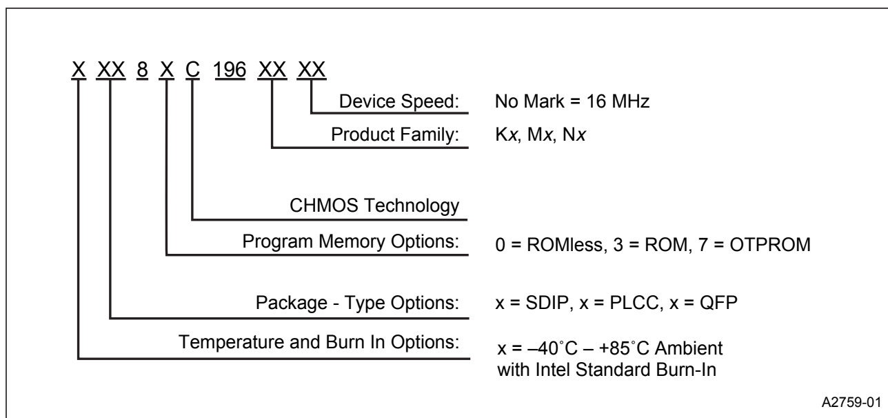
Figure 2. The 8XC196MH Family Nomenclature
