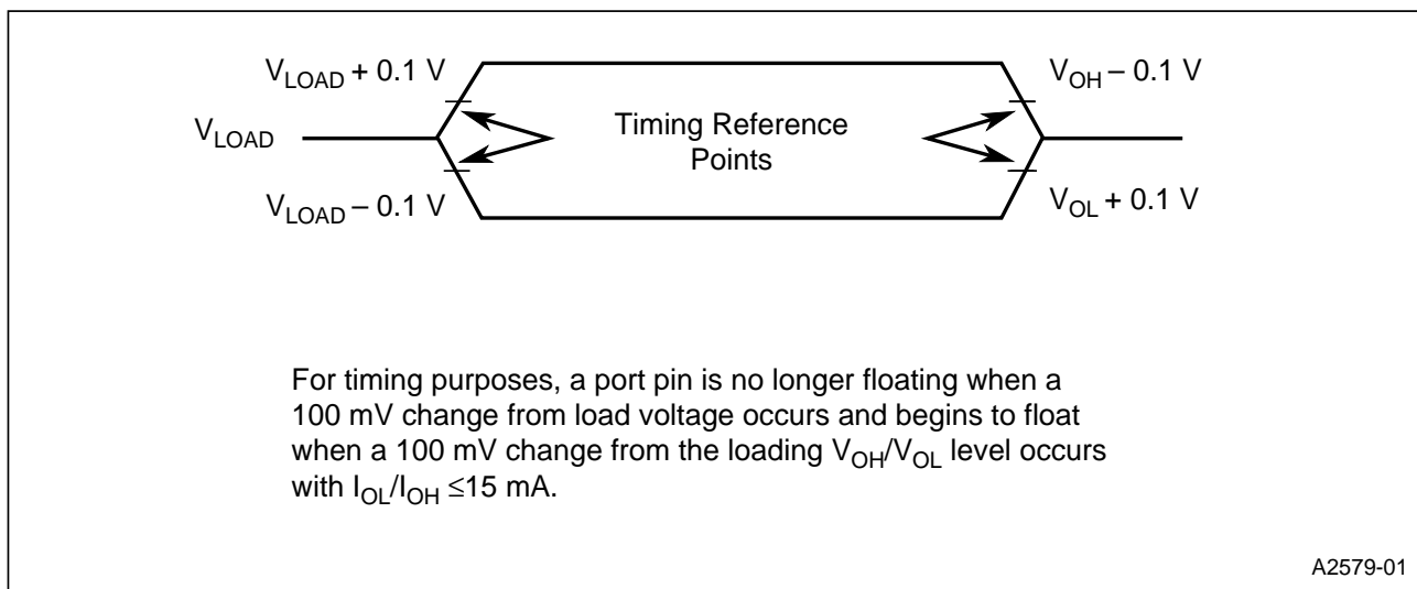
Figure 14. Float Waveforms
