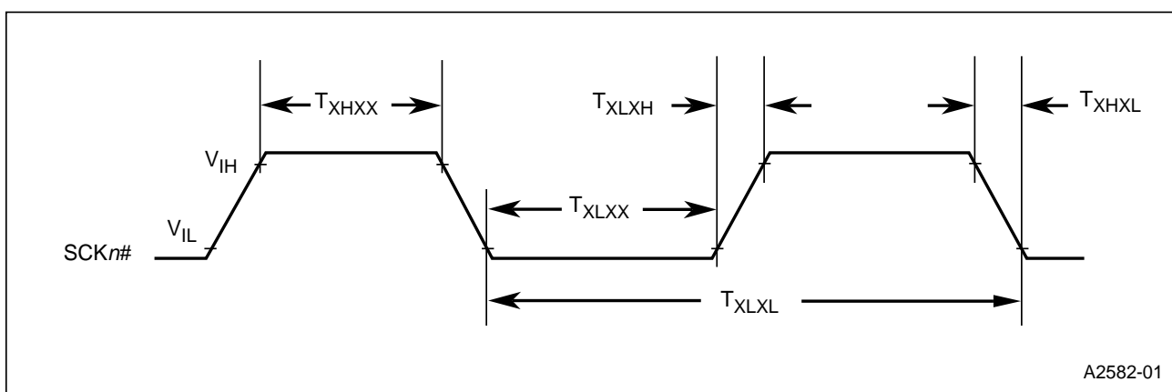
Figure 17. Serial Port Waveform — Clock Drive (DIR = 1)
