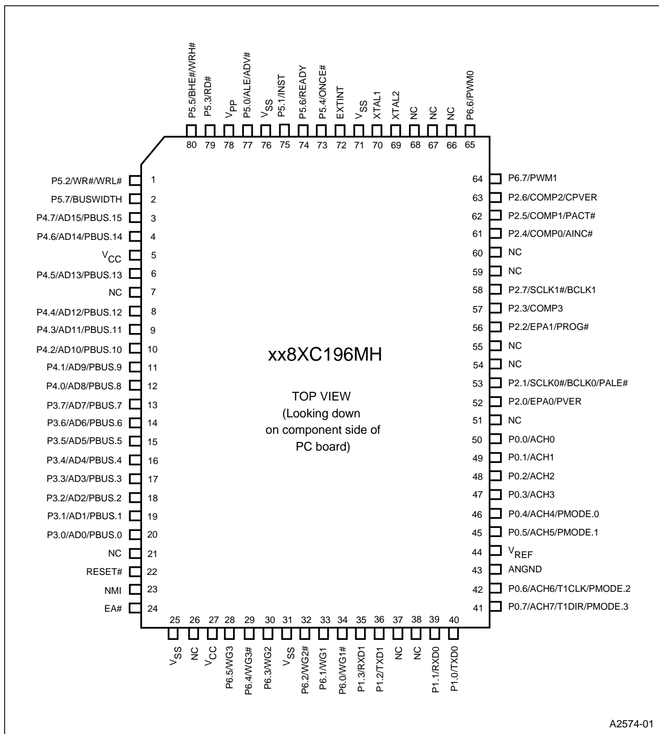
Figure 5. 8XC196MH 80-lead Shrink EIAJ/QFP Package
