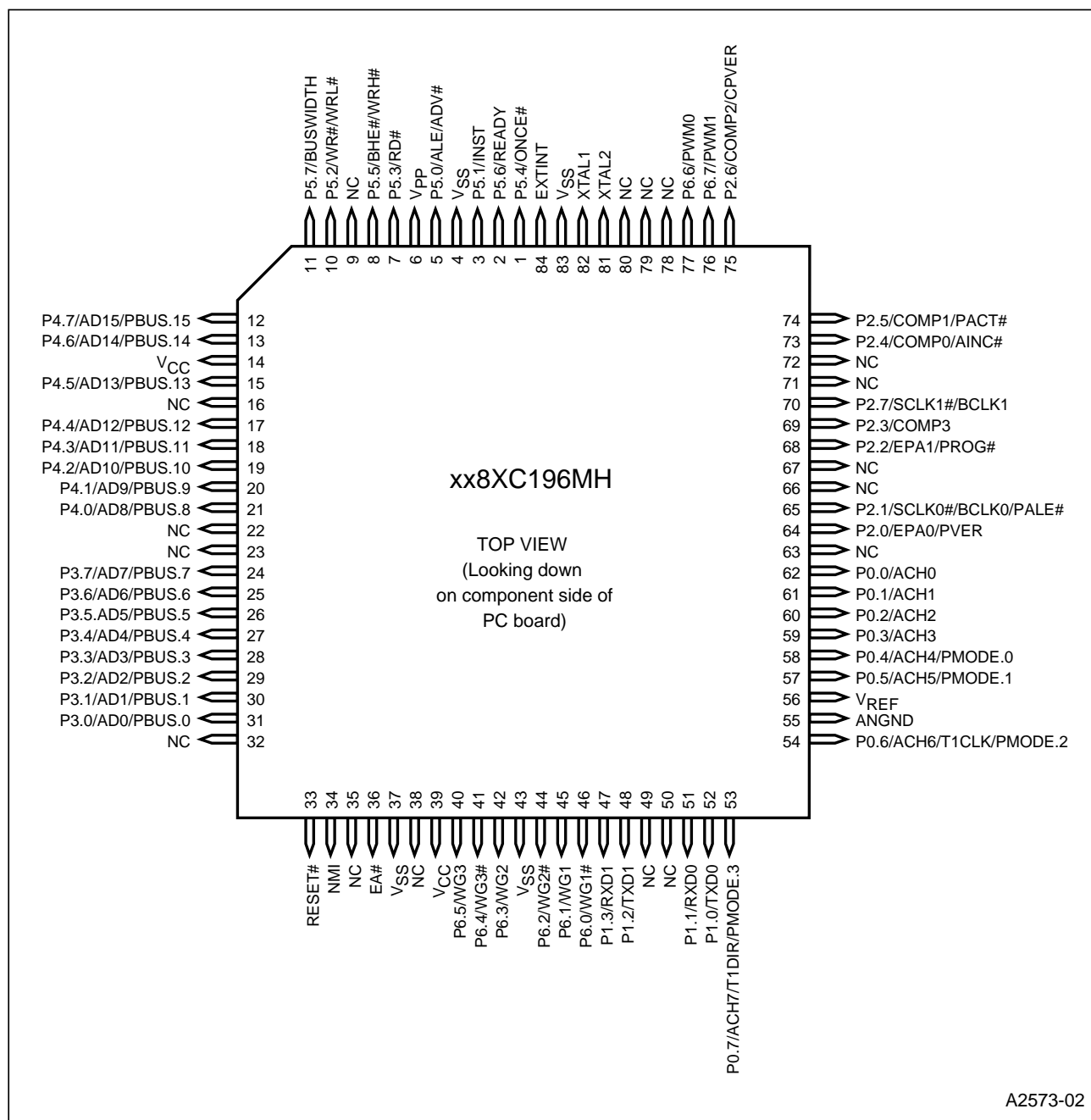
Figure 4. 8XC196MH 84-lead PLCC Package
