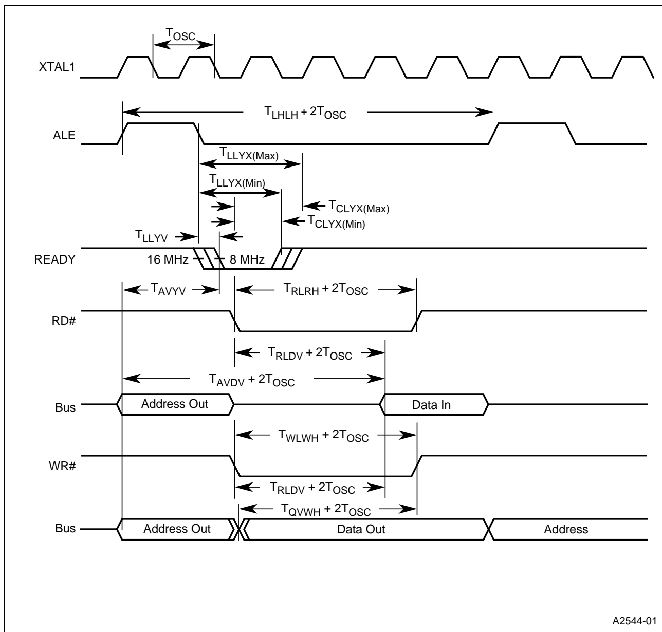
Figure 8. READY Timing Diagram (One Wait State)
