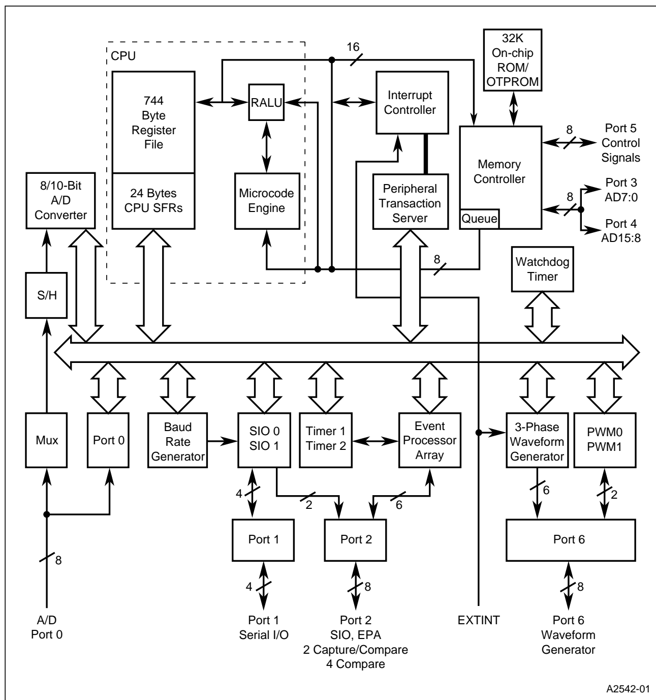
Figure 1. 8XC196MH Block Diagram
