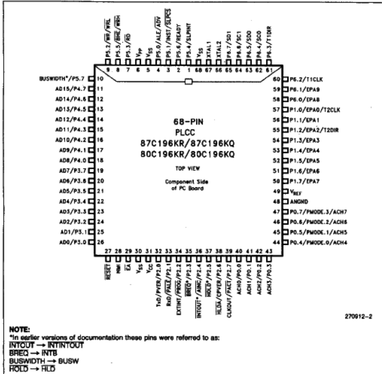
Figure 2. Package Diagrams
