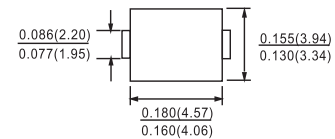
DO-214AA(SMB)
