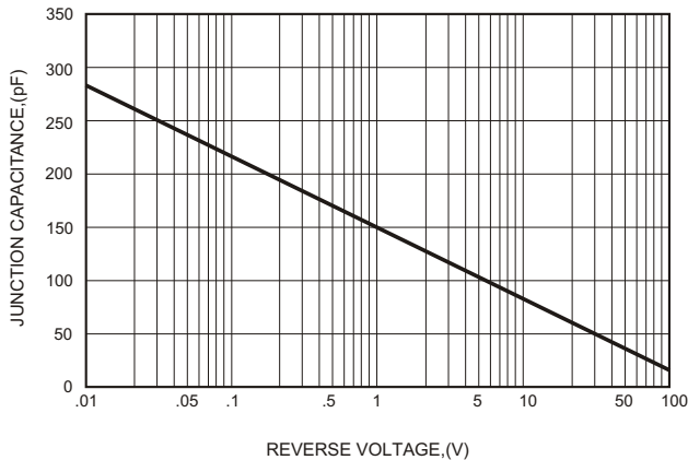
FIG.4-TYPICAL JUNCTION CAPACITANCE
