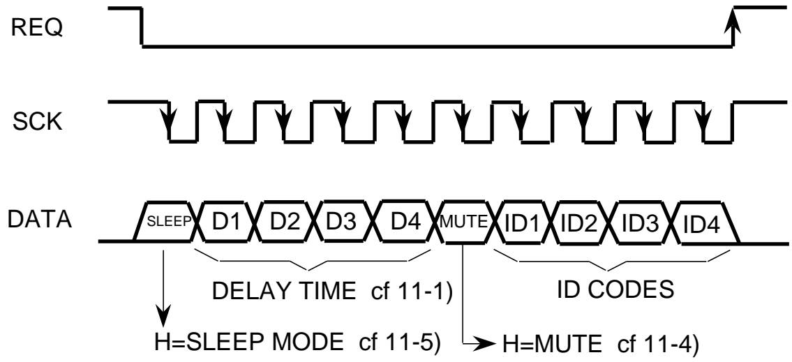
TIMING DIAGRAM
