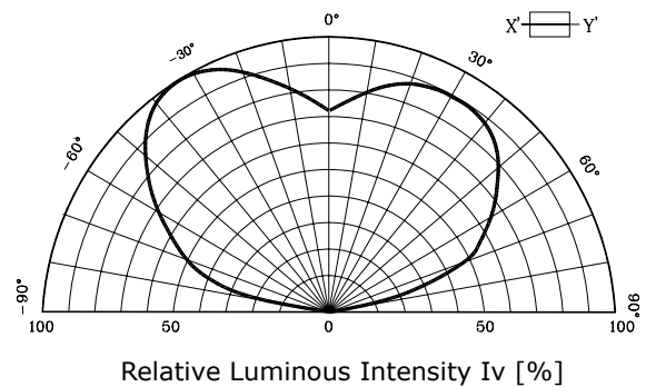
Fig. 5-2 Radiation Diagram(Y)
