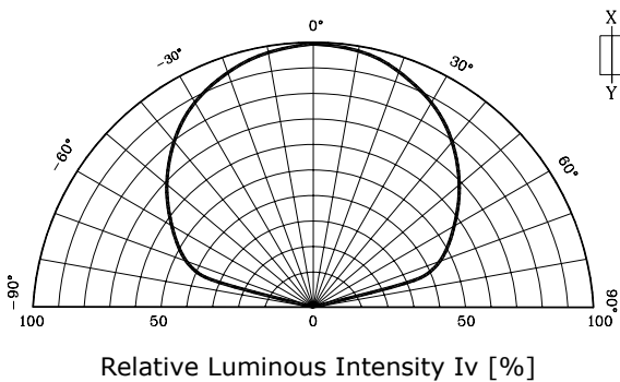
Fig. 5-1 Radiation Diagram(X)
