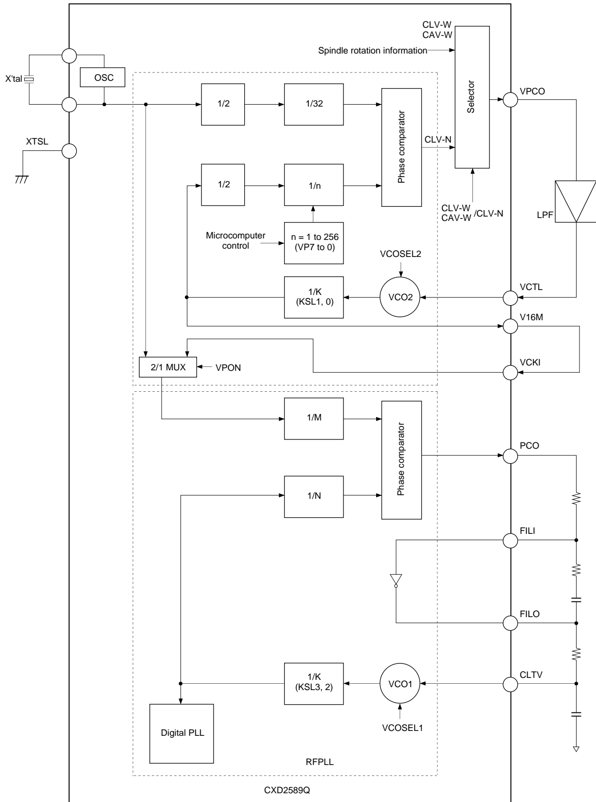
Block Diagram 4-1
