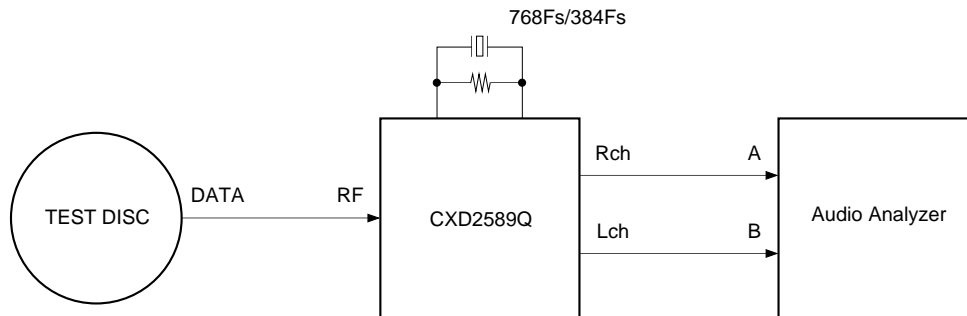
Block Diagram for Measuring Analog Characteristics
