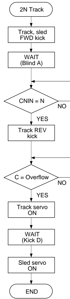
Fig. 4-6-(a). 2N-Track Jump Flow Chart
