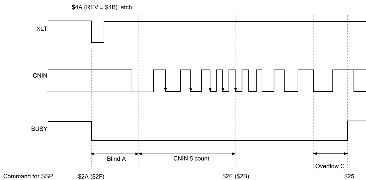
Fig. 4-5-(b). 10-Track Jump Timing Chart
