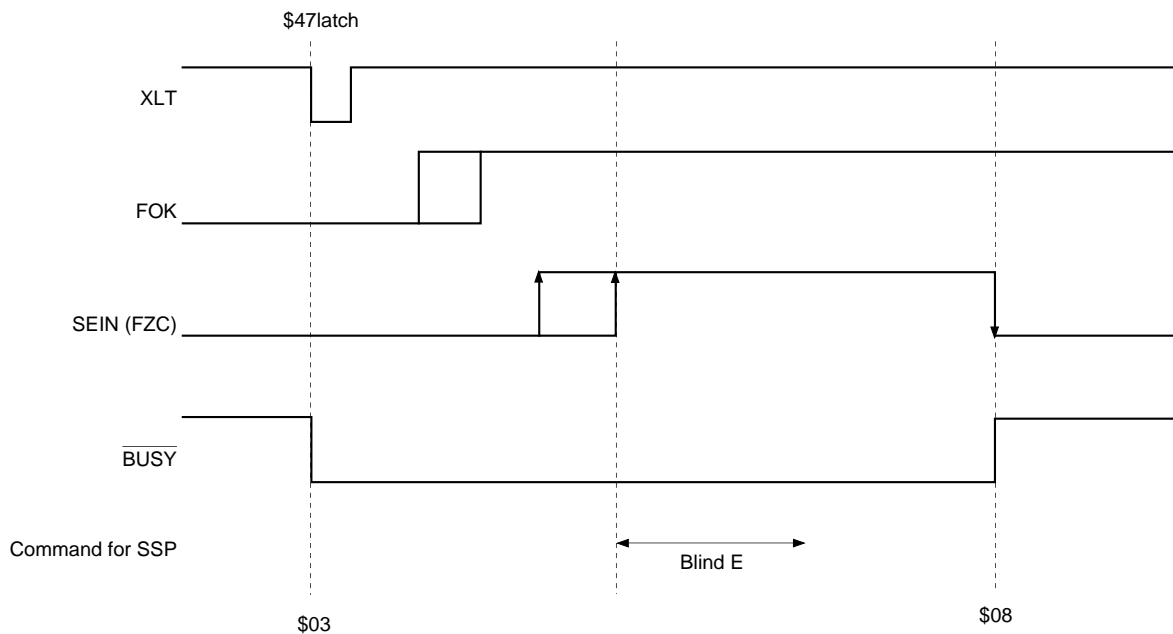
Fig. 4-3-(b). Auto Focus Timing Chart
