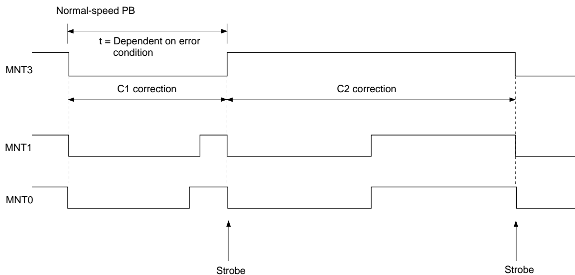
Timing Chart 4-1
