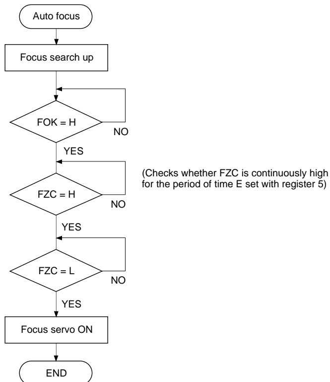
Fig. 4-3-(a). Auto Focus Flow Chart
