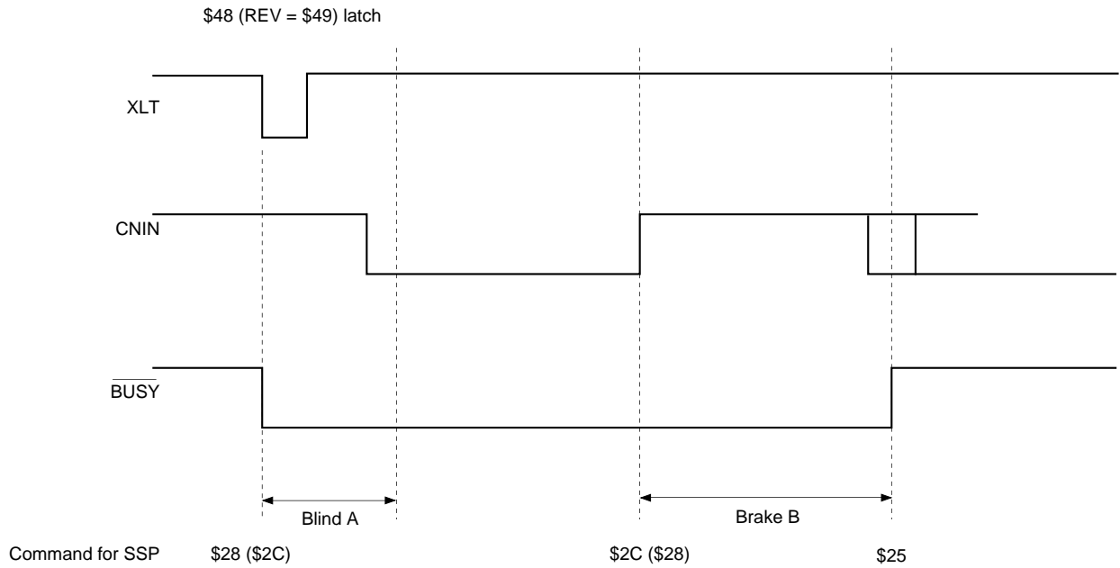
Fig. 4-4-(b). 1-Track Jump Timing Chart
