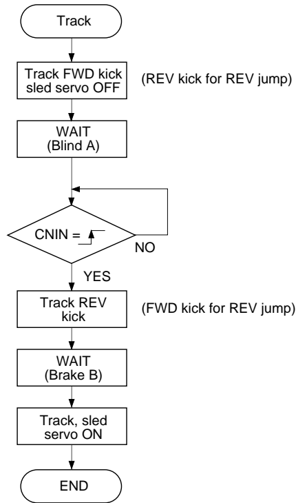
Fig. 4-4-(a). 1-Track Jump Flow Chart
