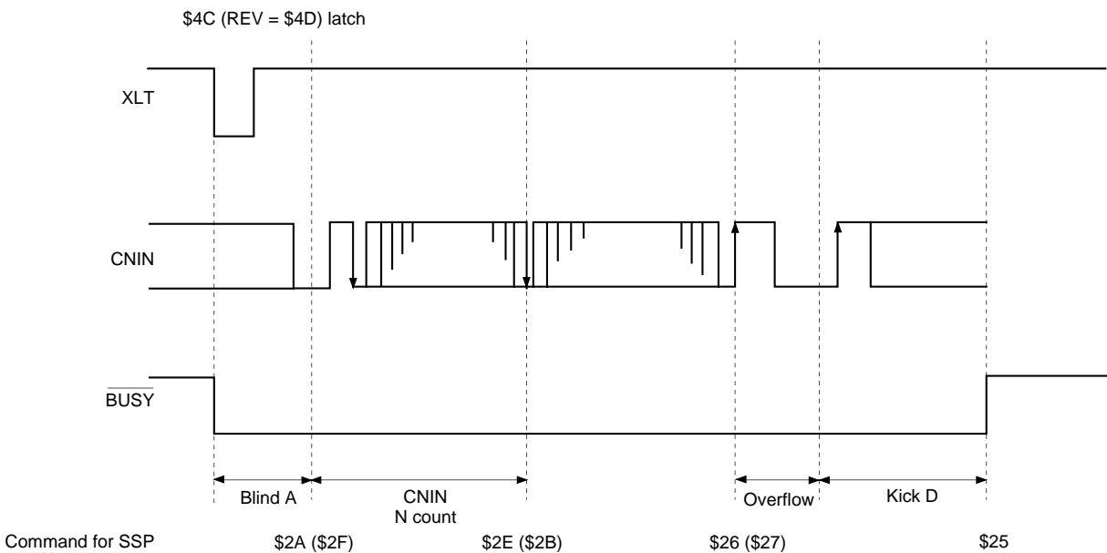
Fig. 4-6-(b). 2N-Track Jump Timing Chart
