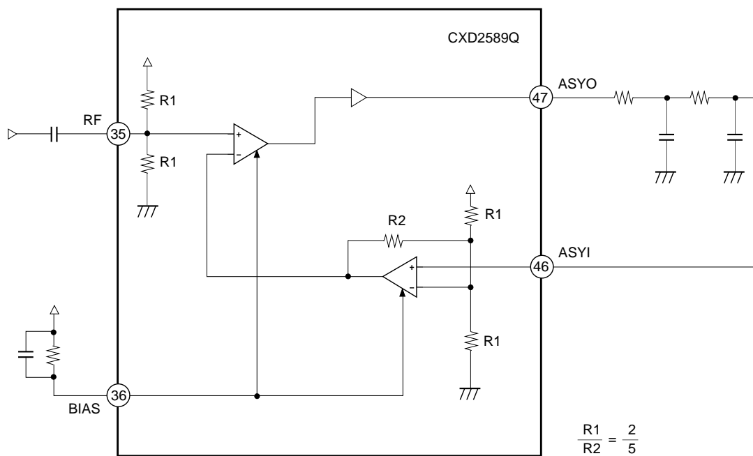
Fig. 4-9. Example of Asymmetry Compensation Application Circuit
