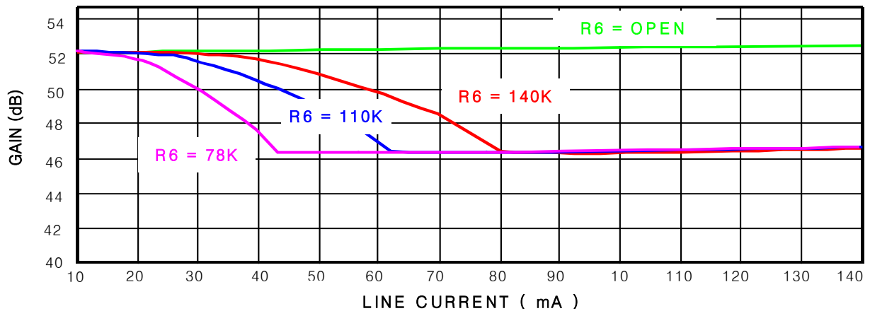
TRANSMIT GAIN V S LINE CURRENT
