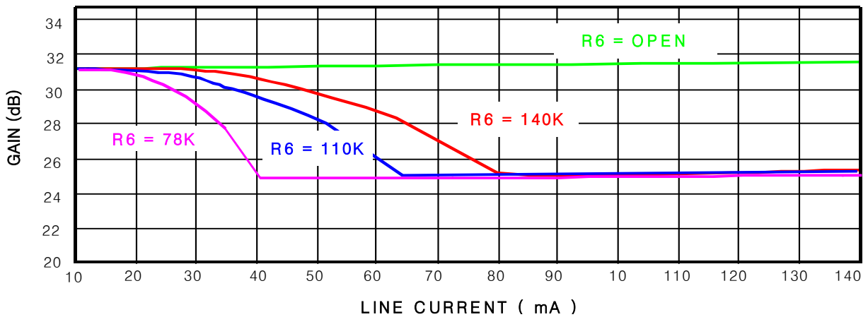
RECEIVE GAIN V S LINE CURRENT
