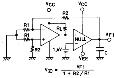
1. Input offset voltage
