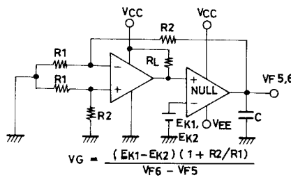
5. Voltage gain
