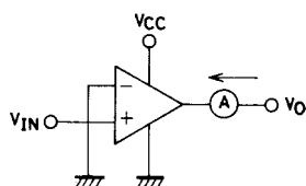
9. Output leakage current
