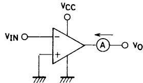
7. Output sink current
