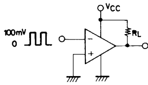
6. Response time
