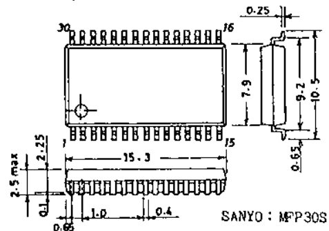
Case Outline 3073A-M30IC [LA7323M] (unit: mm)
