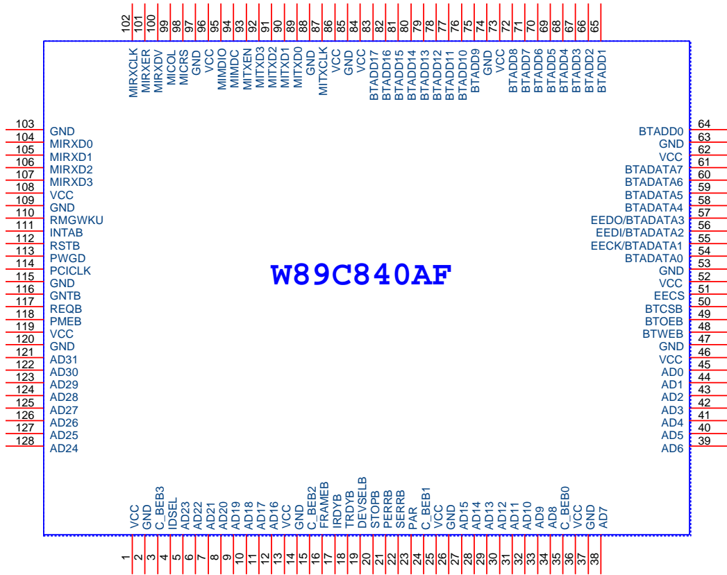
Fig 1: W89C840AF pin configuration
