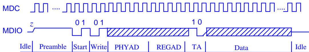
Typical MDIO/MDC Write Cycle
