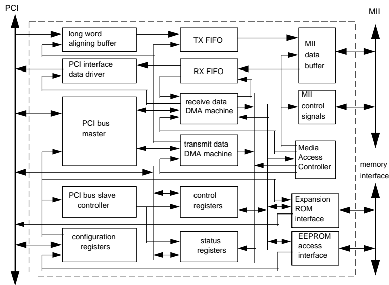
Fig. 2 W89C840AF Block Diagram
