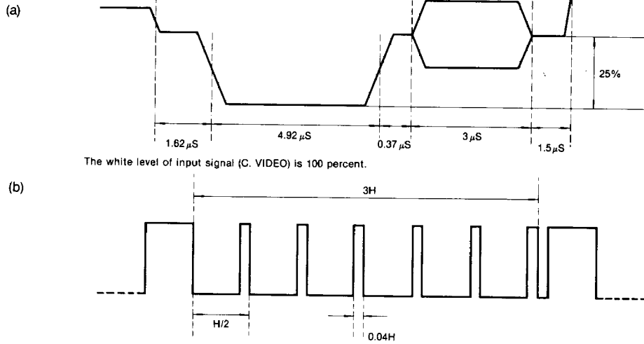
Fig. 3 2V_{pp} Positive composite video signal (a) Horizontal sync pulse. (b) Vertical sync pulse. H equals 63.5 \mu S .
