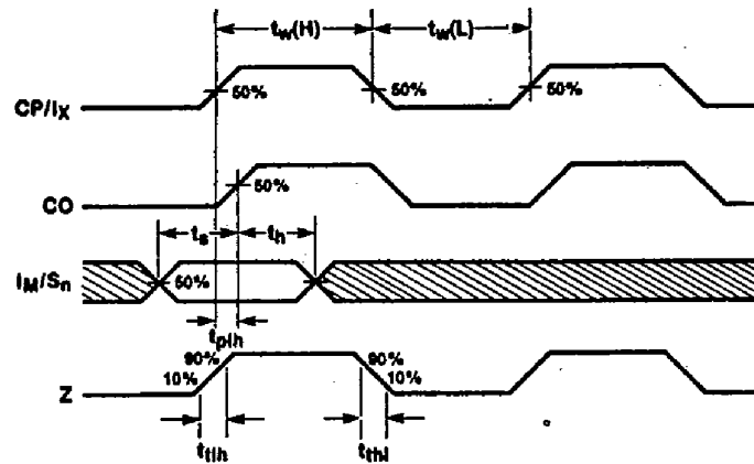
Figure 3: Switching Waveforms
