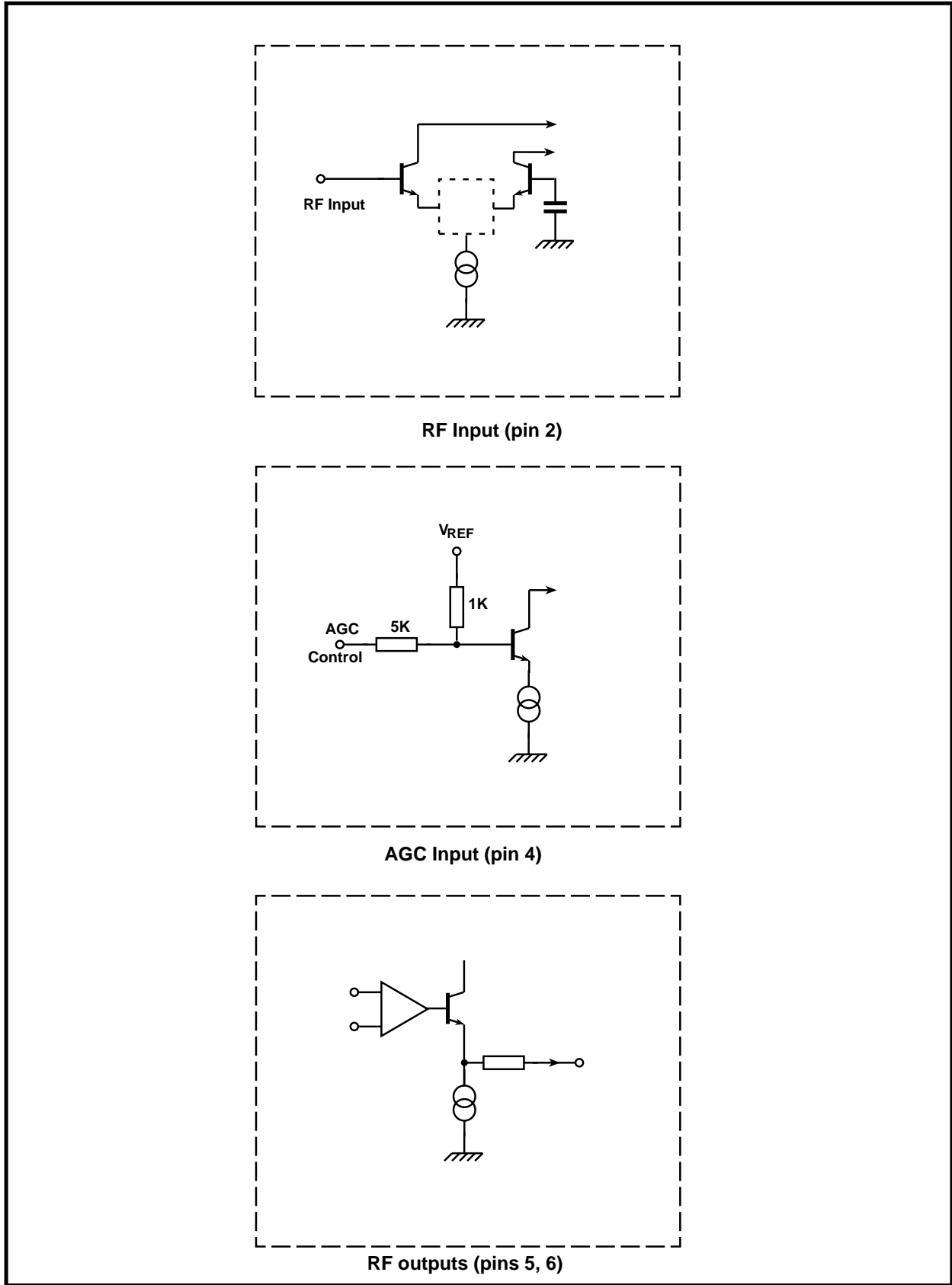
Figure 6 Input/Output interface circuit
