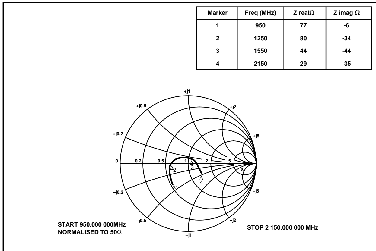
Figure 3 Input impedance (typical)
