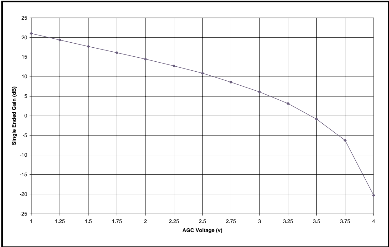
Figure 5 gain variation with AGC voltage (typical)
