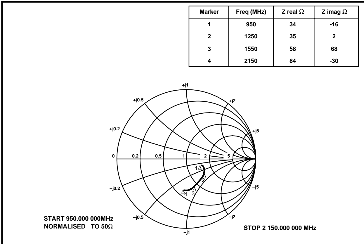
Figure 4 Output impedance (typical)
