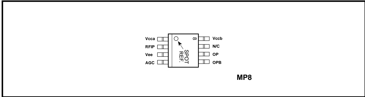
Figure 2 Pin Connections
