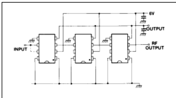
Fig.8 Direct coupled amplifiers
