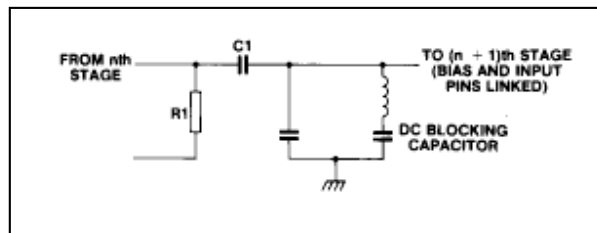
Fig.9 Suitable interstage tuned circuit
