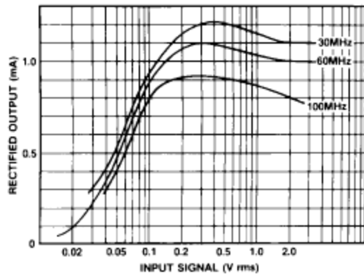
Fig.4 Rectified output current v. input signal
