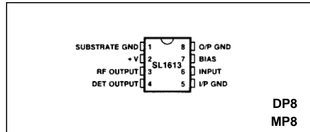
Fig.1 Pin connections (top)
