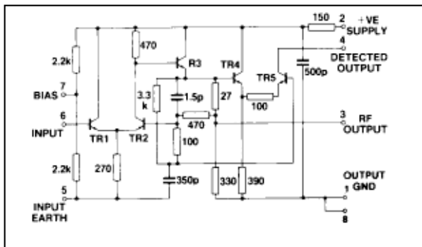
Fig.2 Circuit diagram
