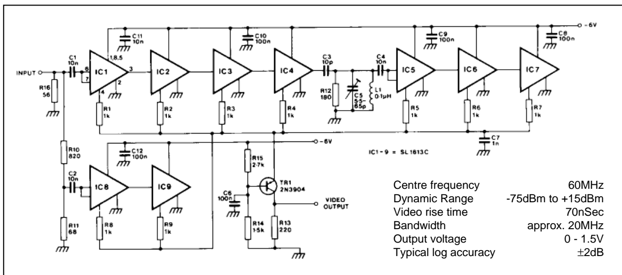
Fig.10 Circuit diagram of low strip
