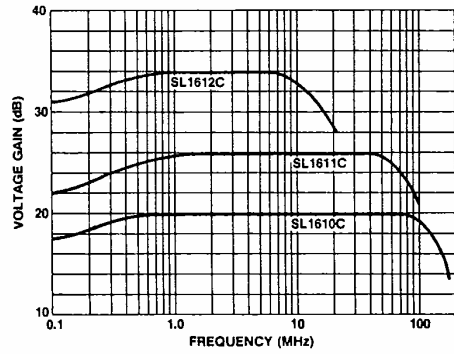
Fig. 8 Typical voltage gain ( R_s=50\Omega )
