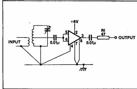
Fig. 7 RF preamplifier
