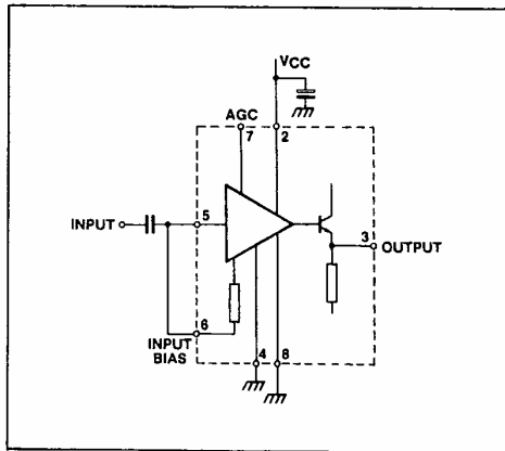
Fig. 2 Block diagram
