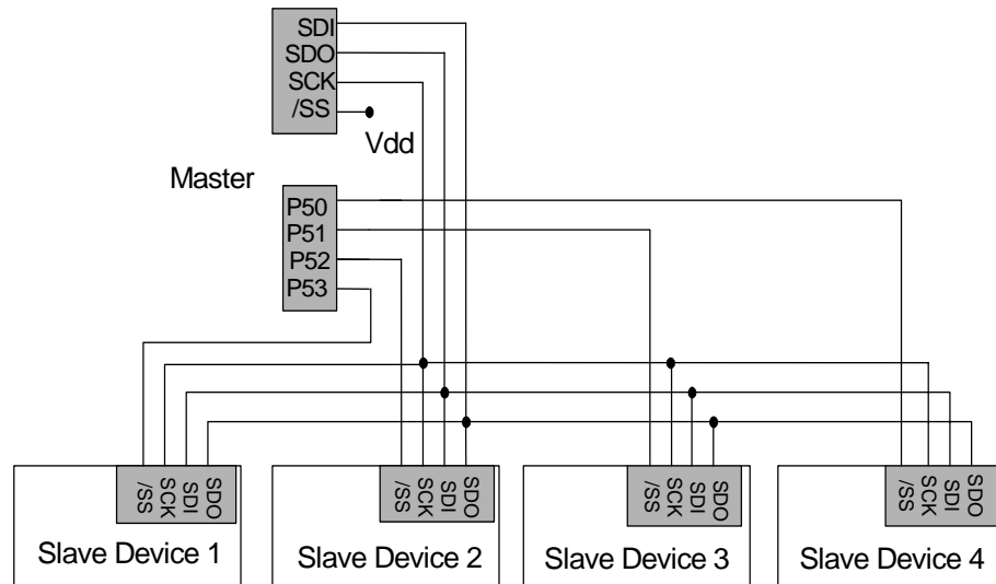
Figure 7-4 SPI Configuration of Single-Master and Multi-Slave
