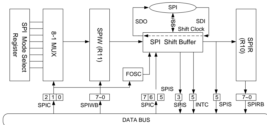
Figure 7-5 Functional Block Diagram of SPI Transmission
