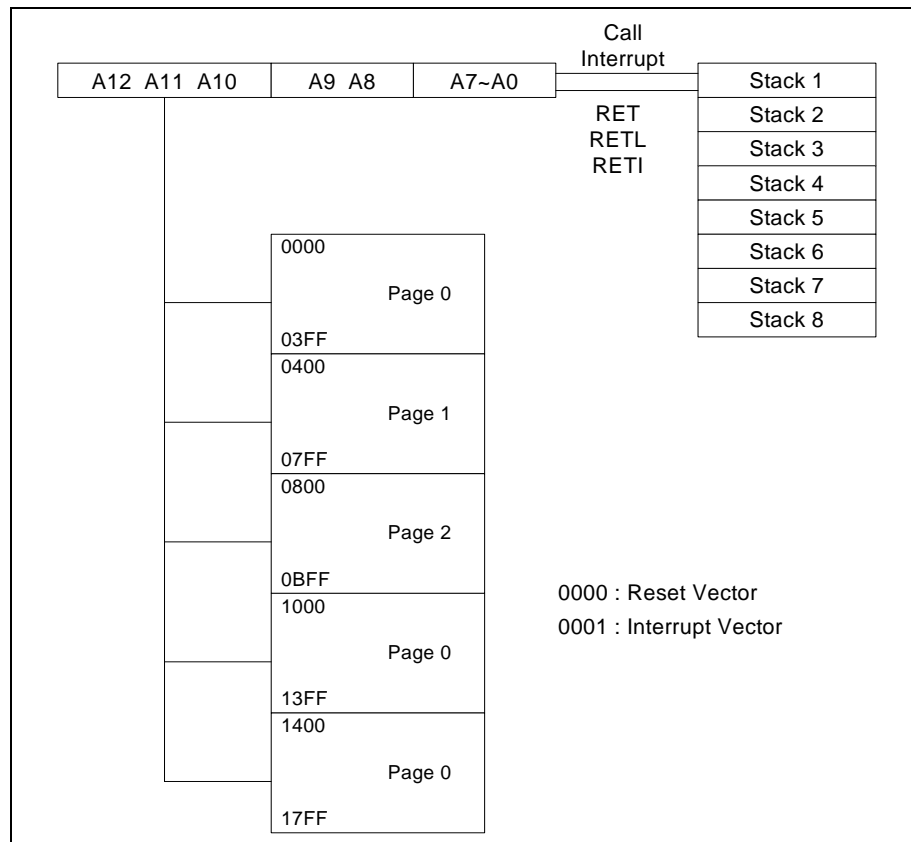
Figure 7-2 Program Counter and Stack
