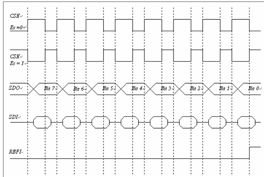
Figure 7-6 SPI Mode with /SS Disabled
