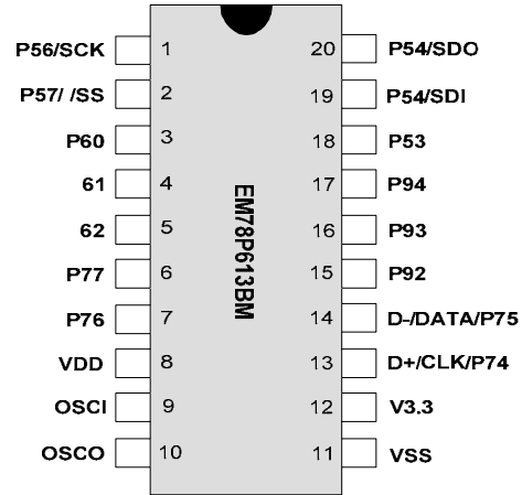
Figure 4-2 EM78P613BM (20-Pin SOP)
