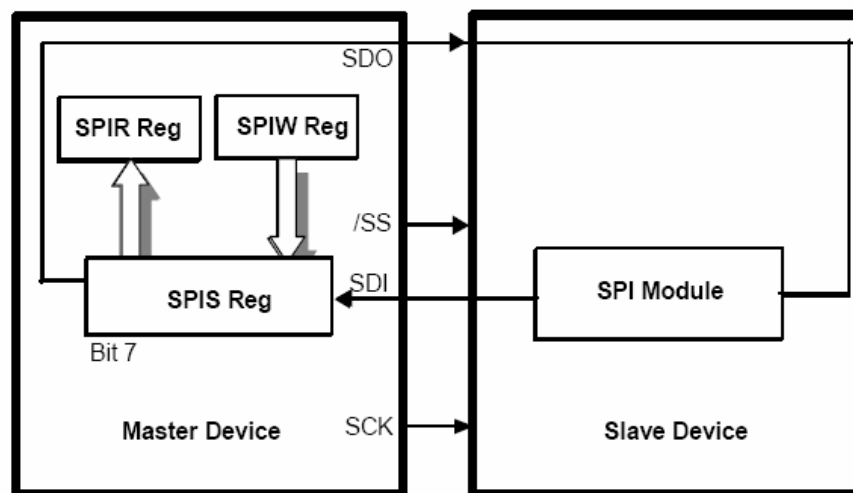
Figure 7-3 SPI Master/Slave Communication
