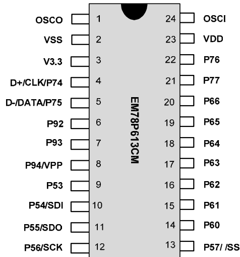
Figure 4-3 EM78P613CM (24-Pin SOP)
