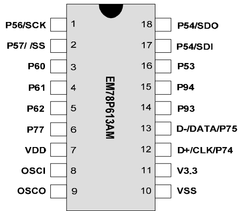
Figure 4-1 EM78P613AM (18-Pin SOP)
