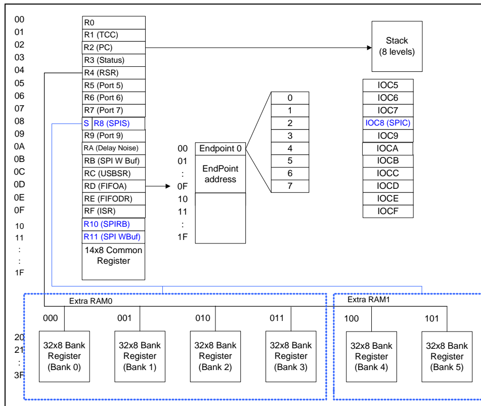
Figure 7-1 Data RAM Organization of EM78P613
