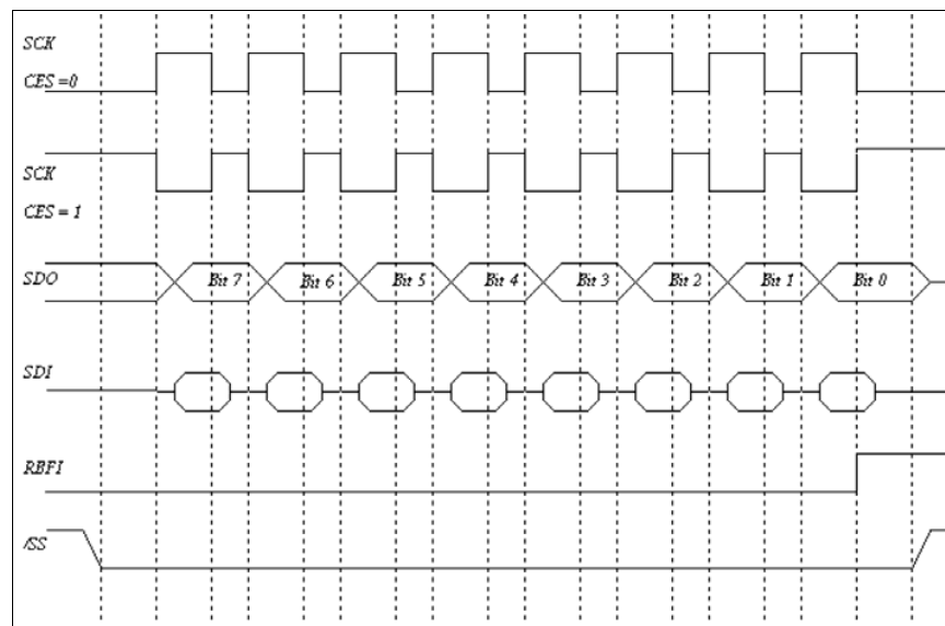
Figure 7-7 SPI Mode with /SS Enabled
